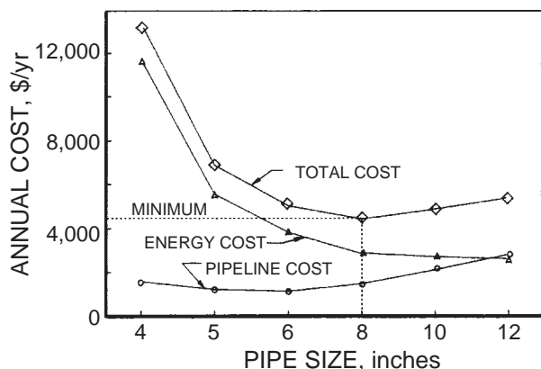
Figure 1.—Annual irrigation cost as varied by mainline pipe size.
