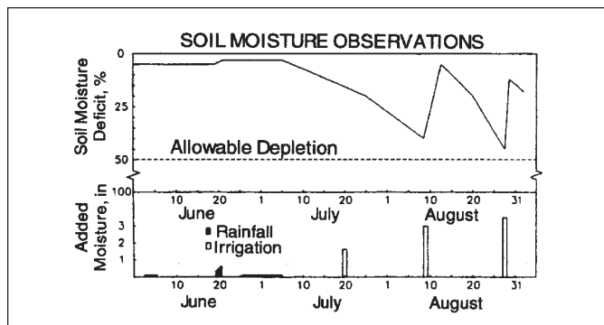
Figure 4.—Typical soil-moisture monitoring chart for a full growing season.
