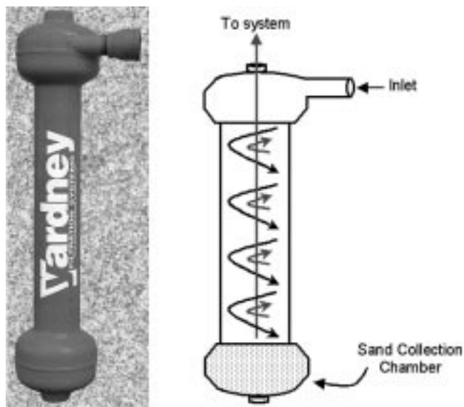
Figure 3. Sand separator (photo courtesy of Yardney Water Management Systems, Inc.)
