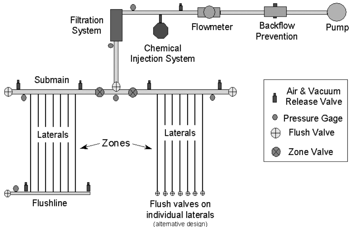
Figure 1. Schematic of micro-irrigation system (courtesy of Kansas State University).
