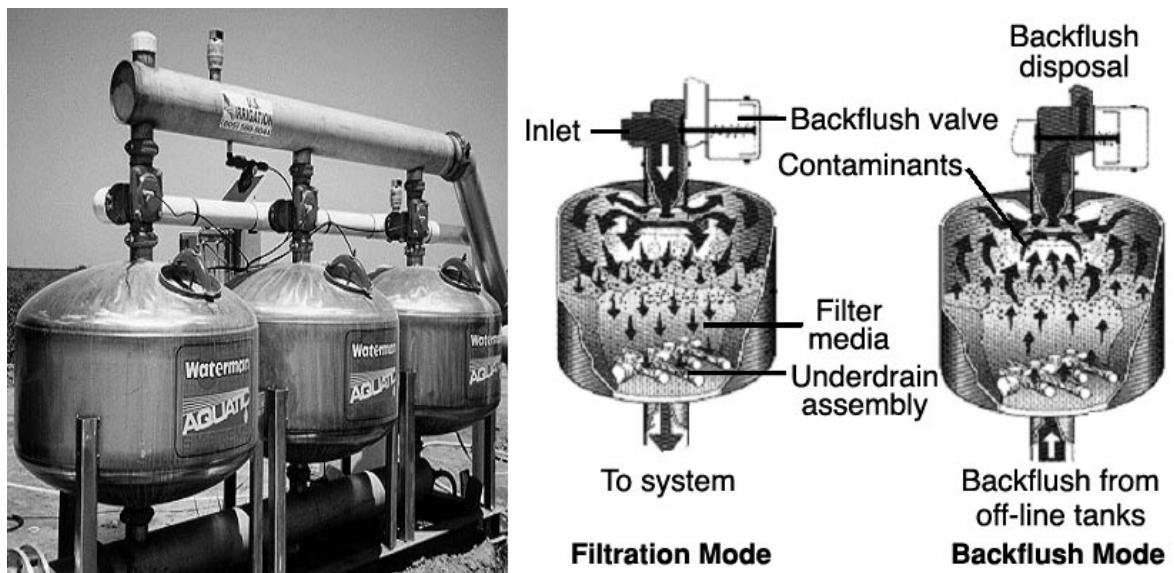
Figure 4. Photo and schematic of sand media filter (photo courtesy of Waterman Industries, schematic adapted from Claude Laval Corp.).
