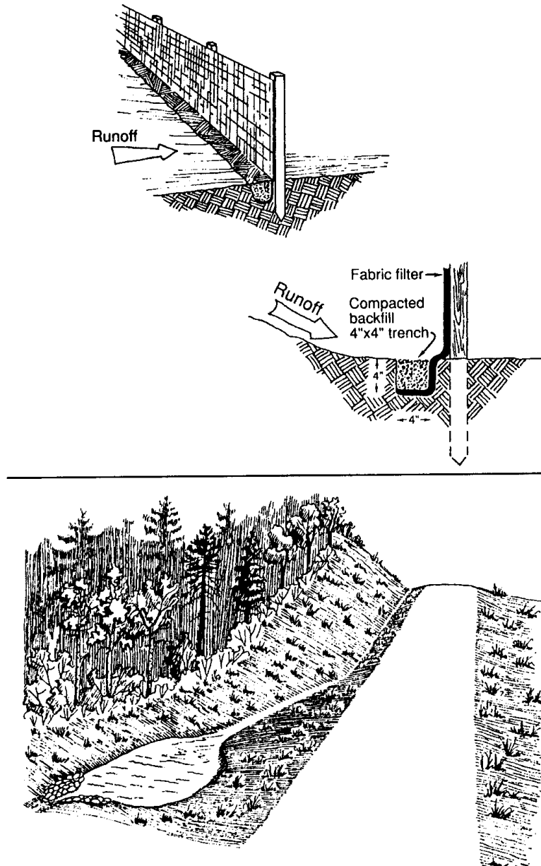
Figure 11.3 A sediment trap to slow runoff and trap sediment for Channelized flow.
