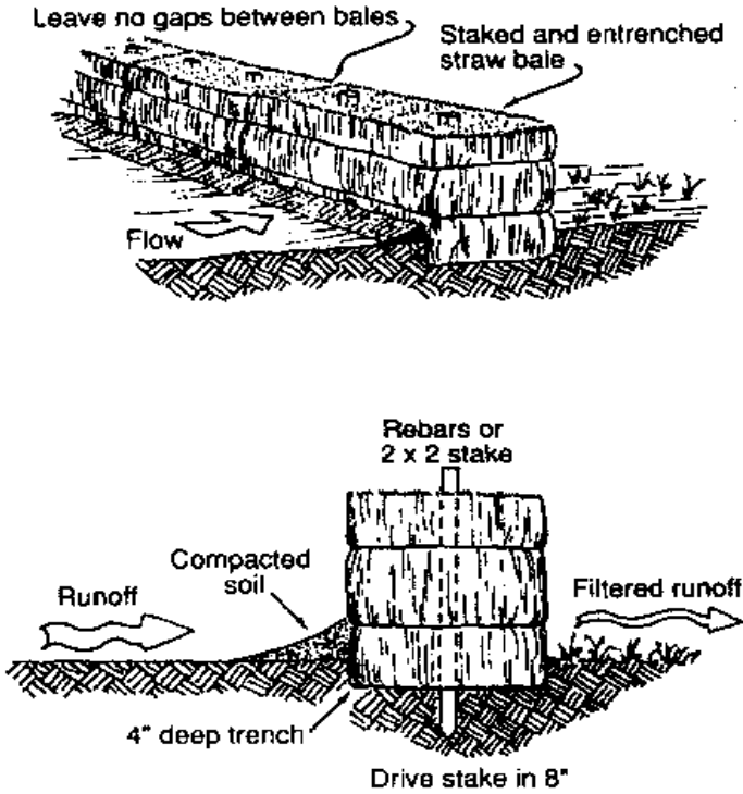
Figure 11.1. Straw bale fencing to slow runoff and trap sediment for sheet flow or channelized flow
