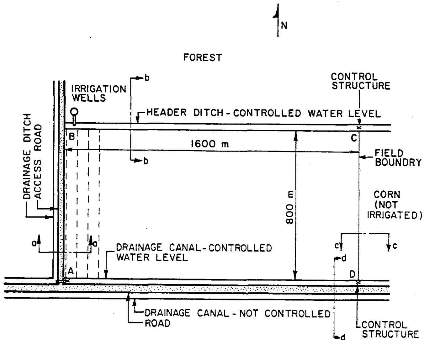
Figure 9-5. Schematic of a 128 ha (307 acre) subirrigation system showing boundary conditions for calculating lateral seepage losses.
