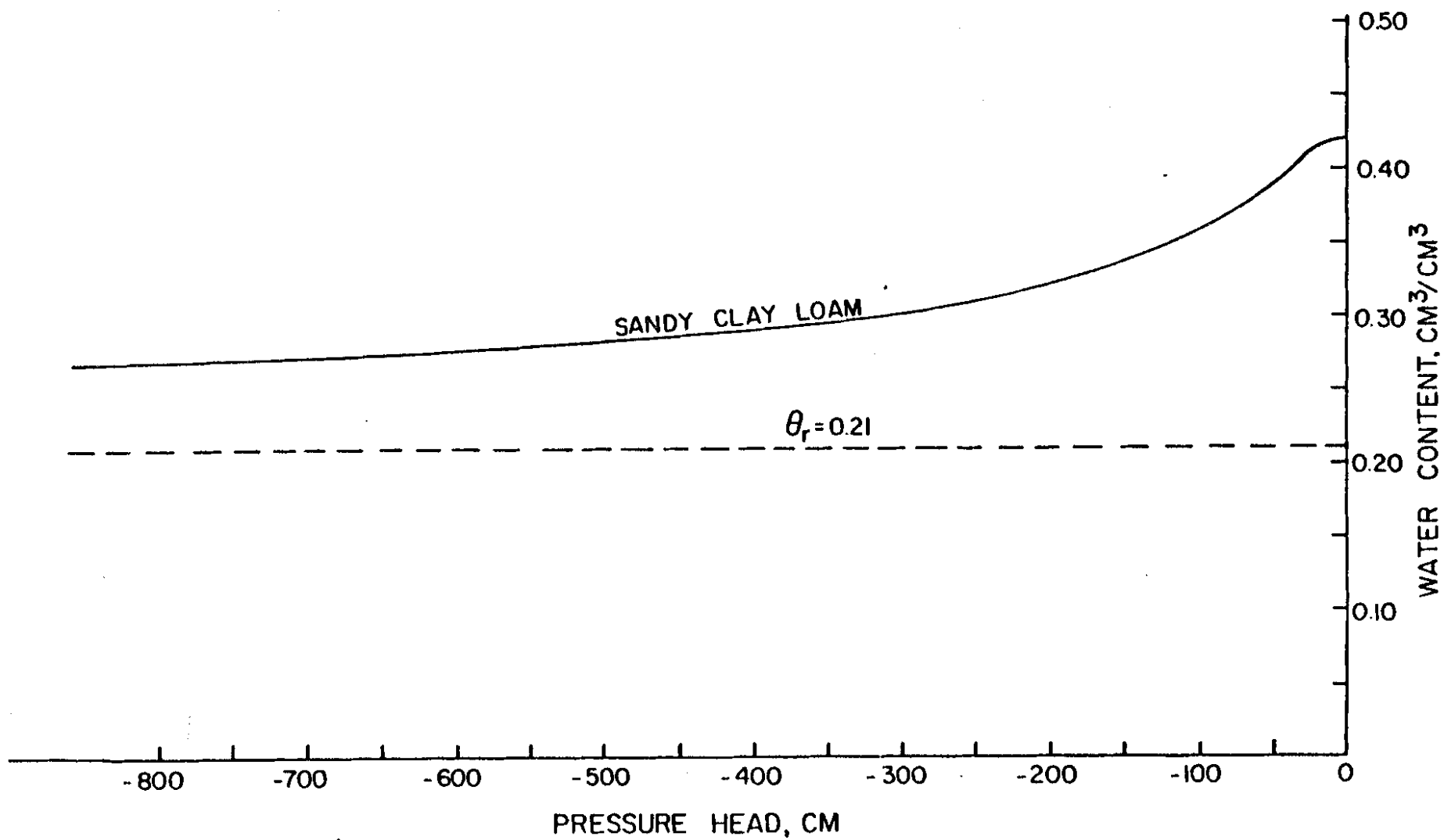
Figure 5-13. Soil water characteristic for a sandy clay loam.
