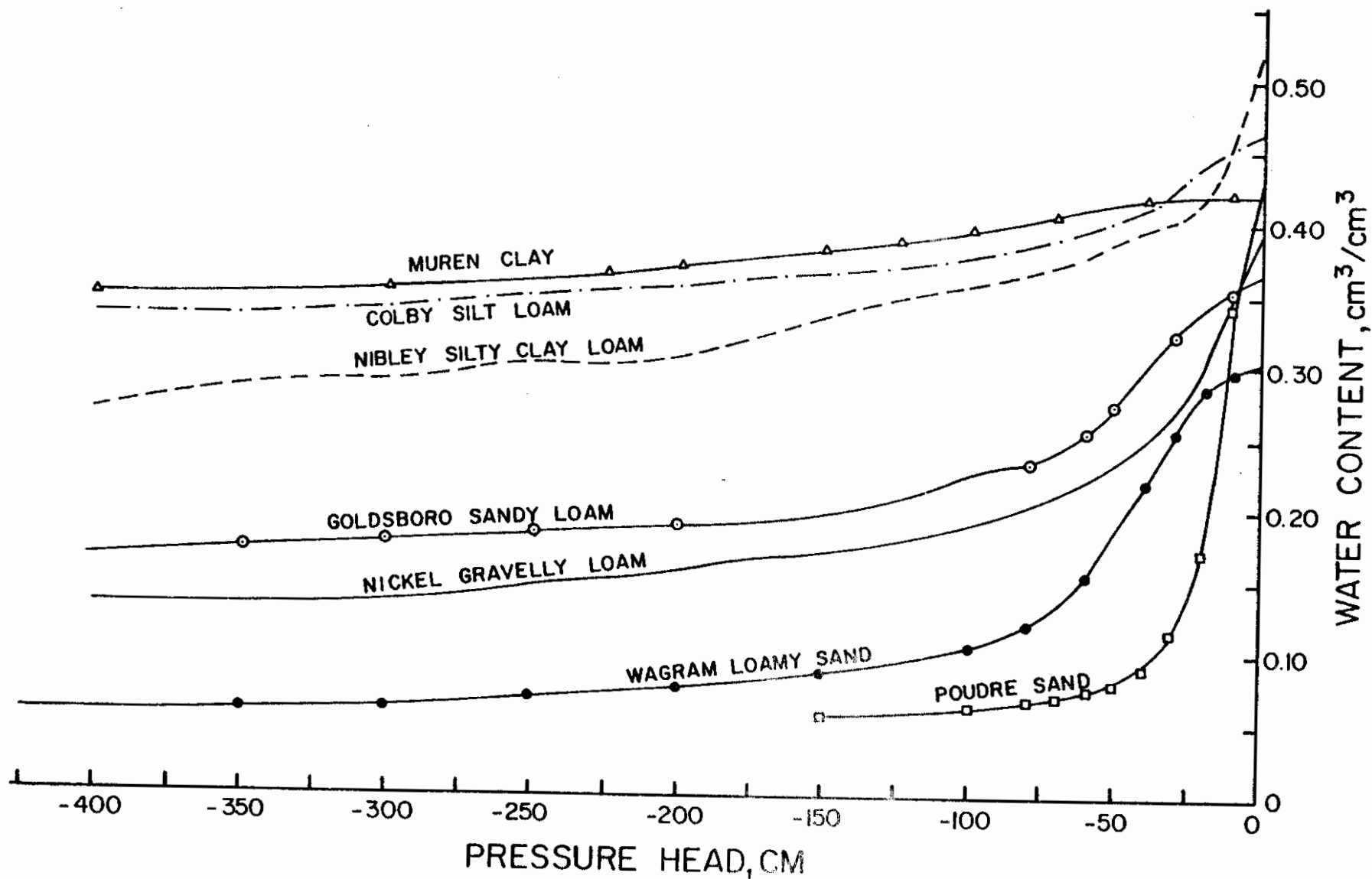
Figure 5-1. Soil water characteristics for 7 soils. Data for the Muren, Colby, Nibley, Nickel and Poudre soils were obtained from Smith (1972). Wagram and Goldsboro data are from Skogerboe (1978).
