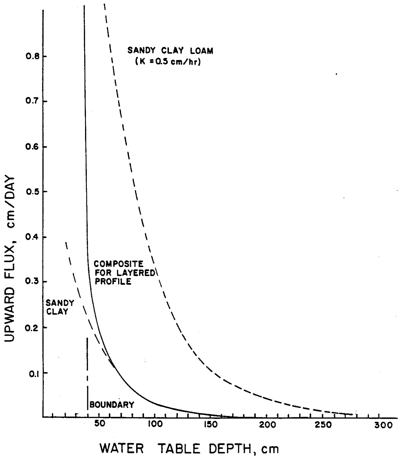
Figure 5-10. Upward flux relationships for a layered profile. The curves were approximated using the relationships in Figure 5-9, as explained in the example.
