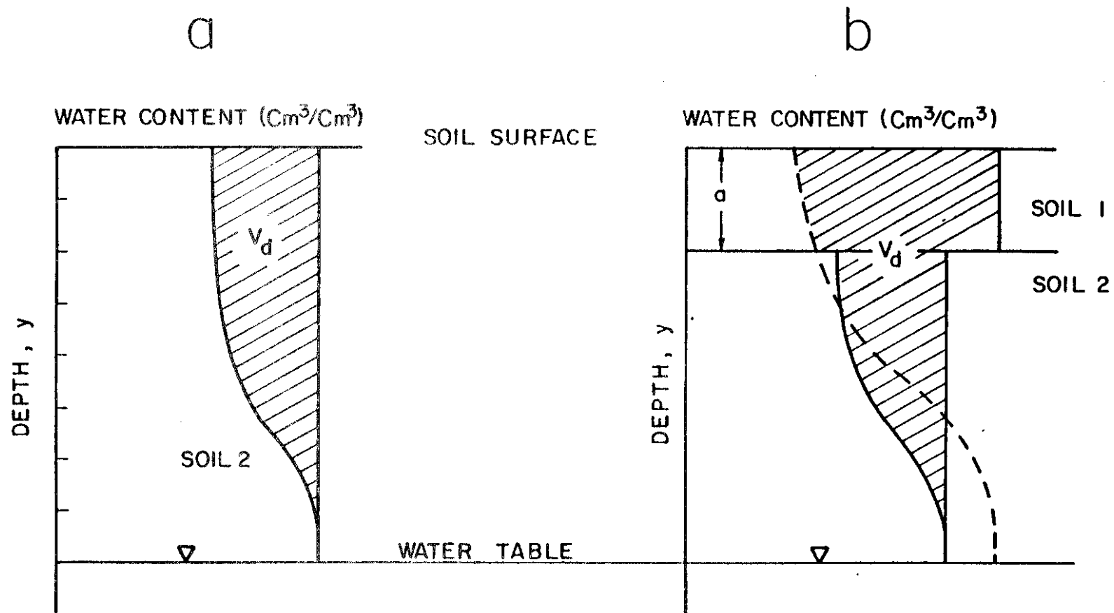
Figure 5-3. Soil water distribution for a uniform soil [a] and a layered soil [b] drained to equilibrium to a water table. The broken curve in [b] represents the soil water distribution for a uniform soil 1.
