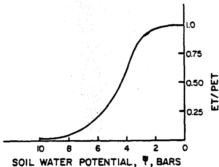
Figure 2-16. Schematic of relative evapotranspiration (ET/PET), as affected by soil water potential, \psi , in the root zone.
