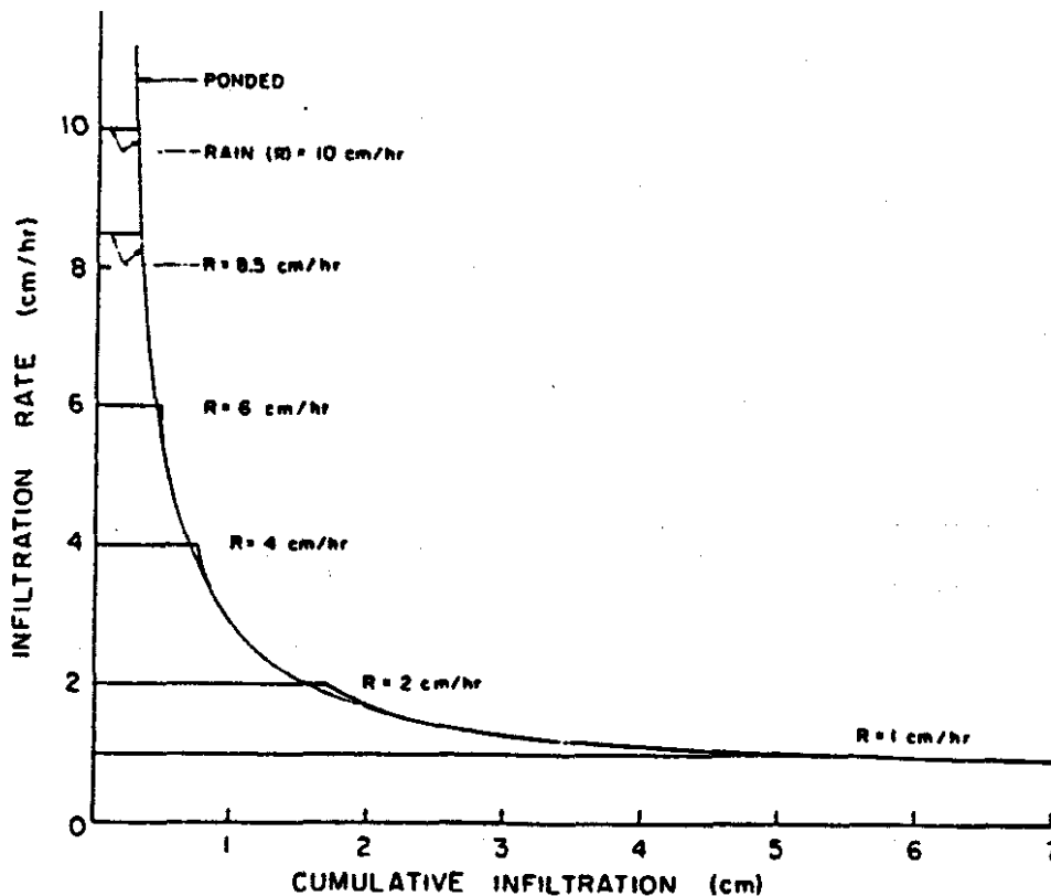
Figure 2-6. Infiltration rate - cumulative infiltration relationships as affected by rainfall rate for the same conditions as Figure 2-5.
