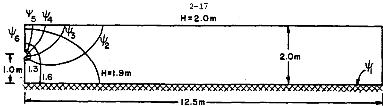
(a) DRAINAGE FROM A PONDED SURFACE
