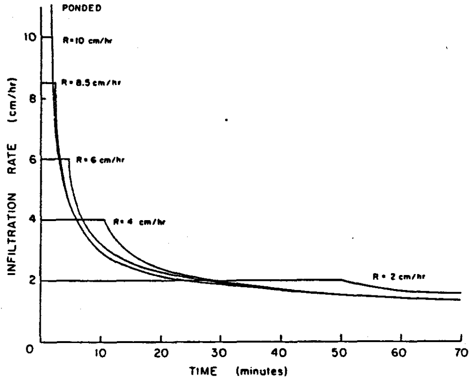
Figure 2-5. Infiltration rate versus time for a sandy loam soil initially drained to equilibrium to a water table 1.0 m deep. Note that the infiltration-time relationships are dependent on the rainfall rate.
