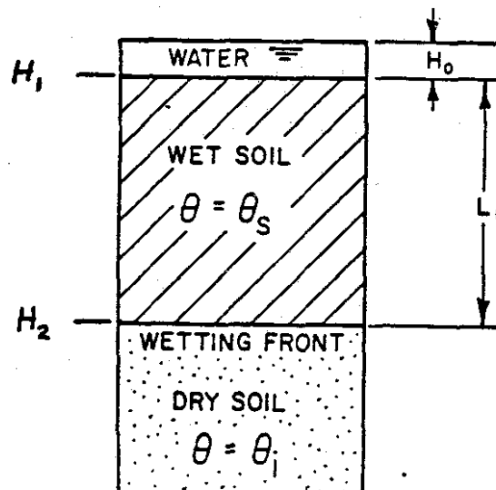
Figure 2-4. Definition sketch for derivation of the Green-Ampt equation.
