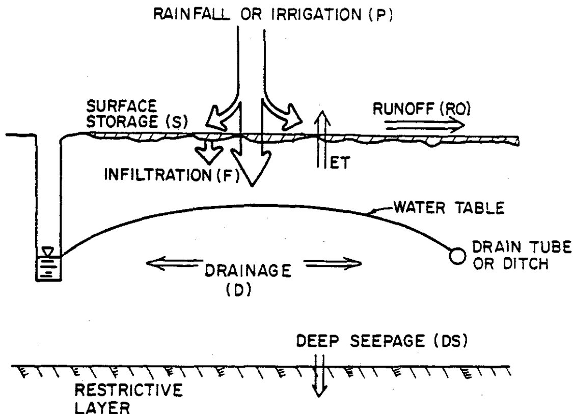
Figure 2-2. Schematic of water management system with drainage to ditches or drain tubes. Components considered in the water balance are shown on the diagram.
