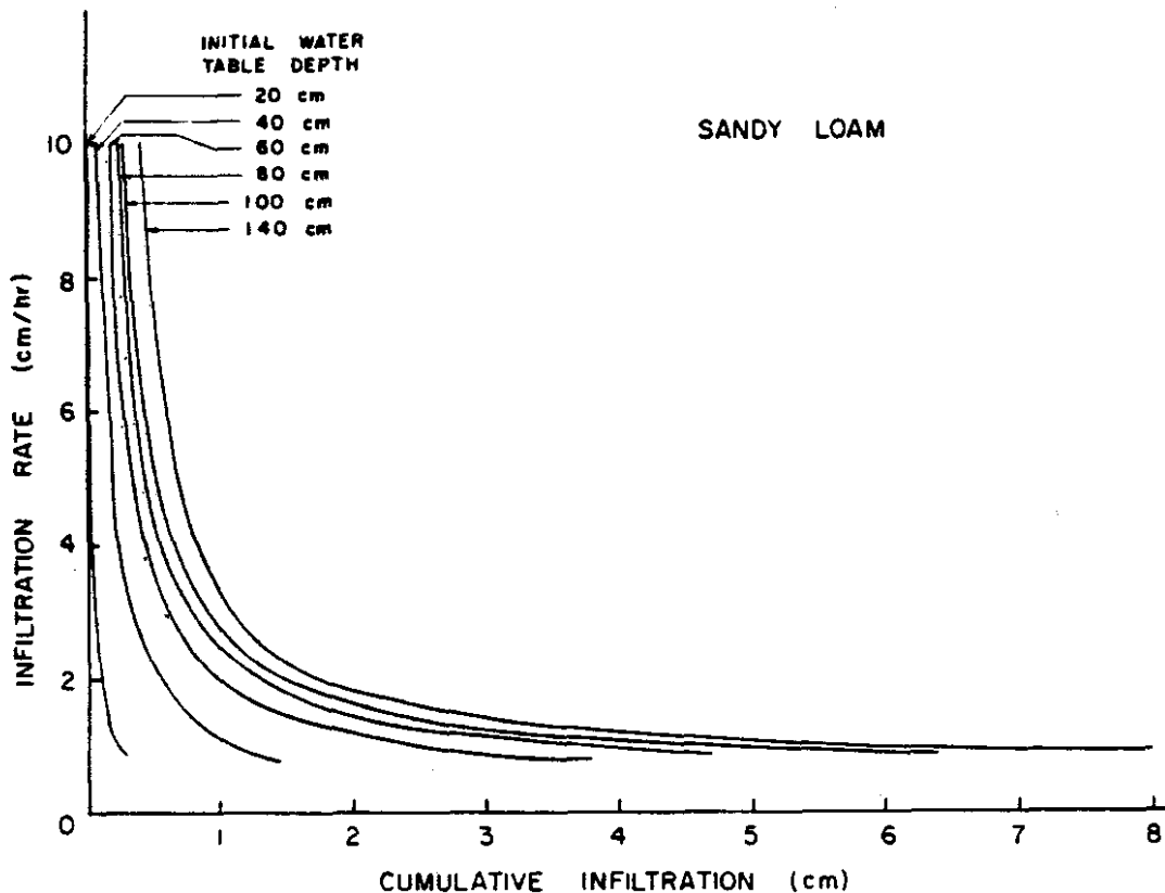
Figure 2-7. Infiltration relationships for the sandy loam soil of Figure 2-5 initially drained to equilibrium at various water table depths.
