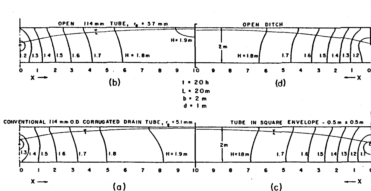
Figure 2-9. Water table position and hydraulic head, H , distribution in a Panoche soil after 20 hours of drainage to (a) conventional 114 mm (4-inch) drain tubes; (b) wide open (no walls) 114 mm diameter drain tubes; (c) a drain tube in a square envelope 0.5 m x 0.5 m; and (d) an open ditch 0.5 m wide. The drain spacings in all cases were 20 m. (After Skaggs and Tang, 1978).
