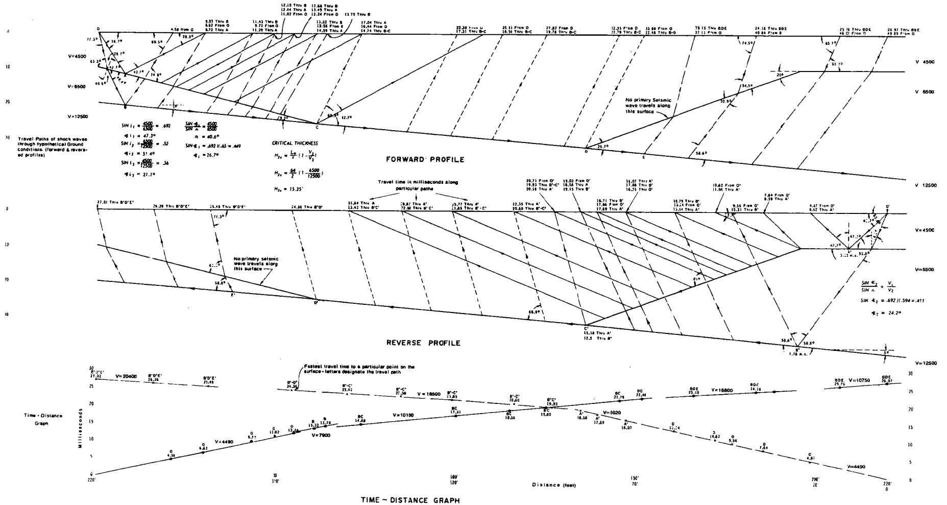
Figure 2-32. - Computed Seismogram.
