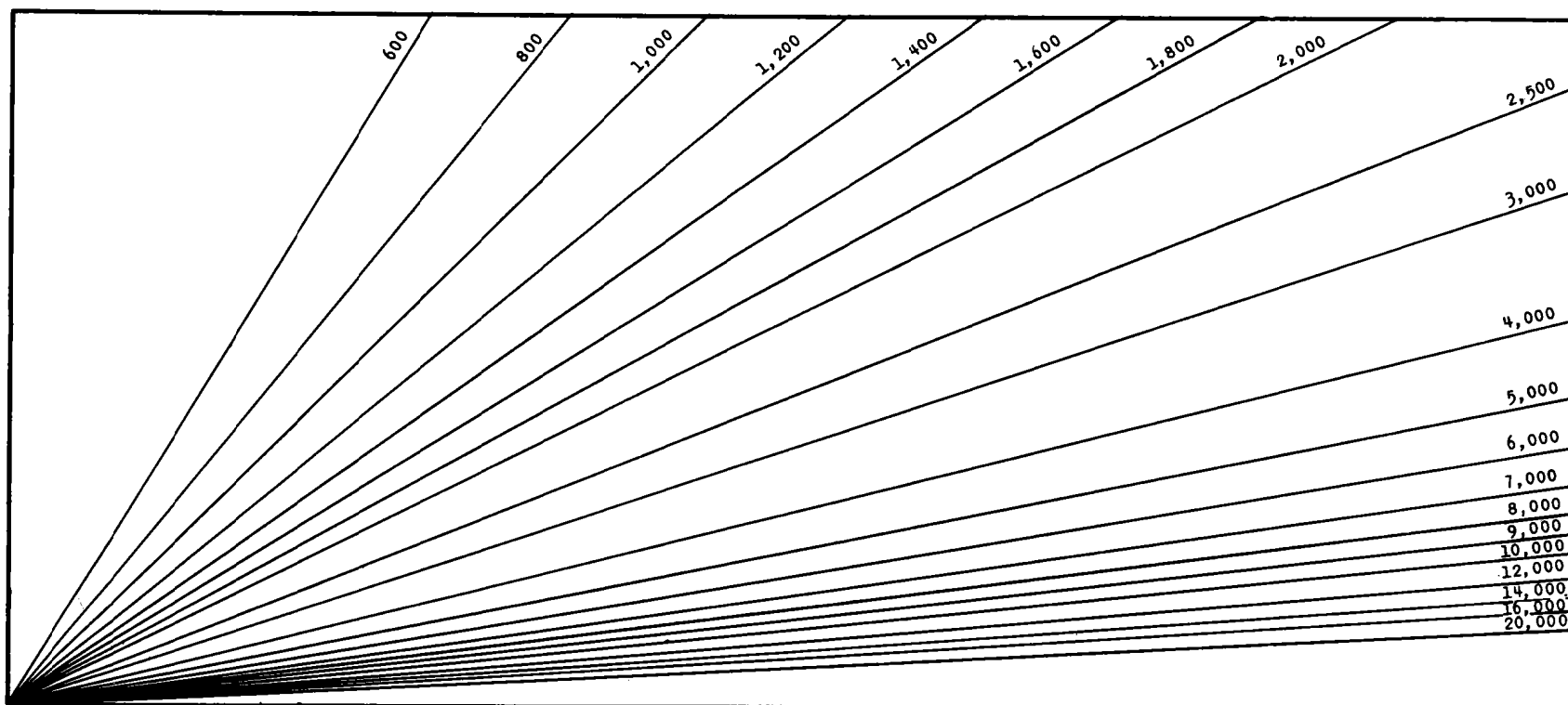
Figure 2-9. — Velocity overlay
