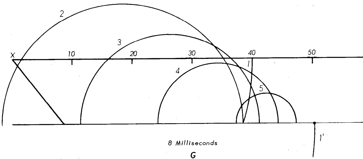
Figure 2-2. — Refracted Waves. (Continued)
