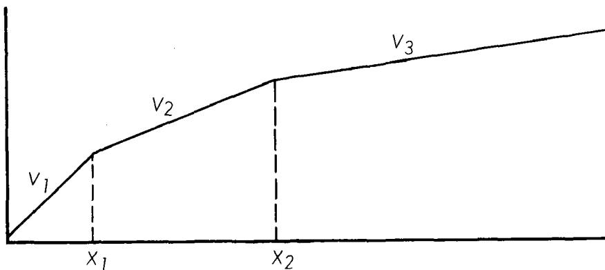
Figure 2-10. - Critical Distances.
