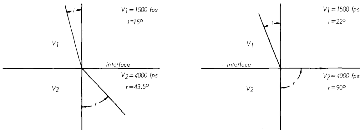
Figure 2-1. - Snell's Law.
