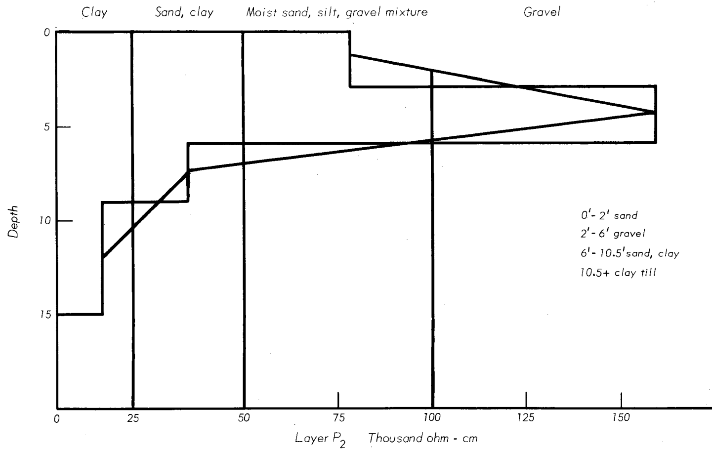
Figure 3-16. — Barnes Layer Method
