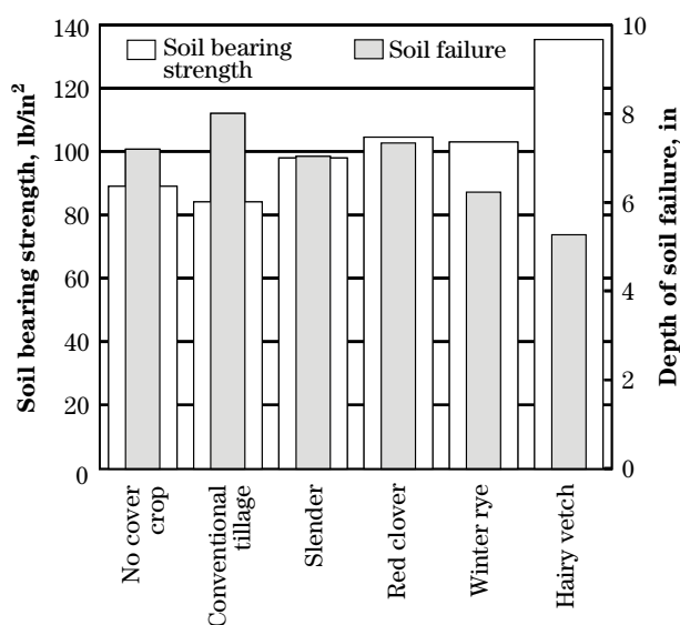
Figure 6 Bearing strength of soil (Osborne et al. 2002)
