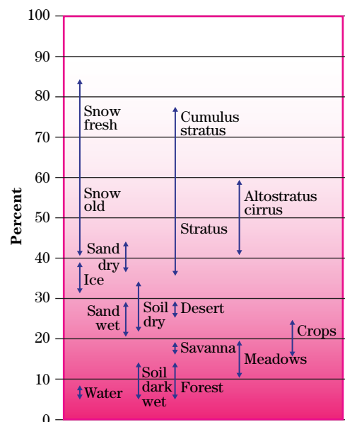
Figure 1 Percentage of diffusely reflected sun light in relation to various surface conditions of the earth (Grobe 2006)
