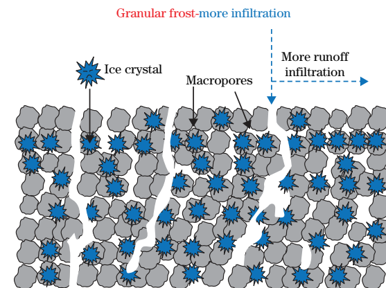
Figure 3 Conceptual diagram of granular frost
