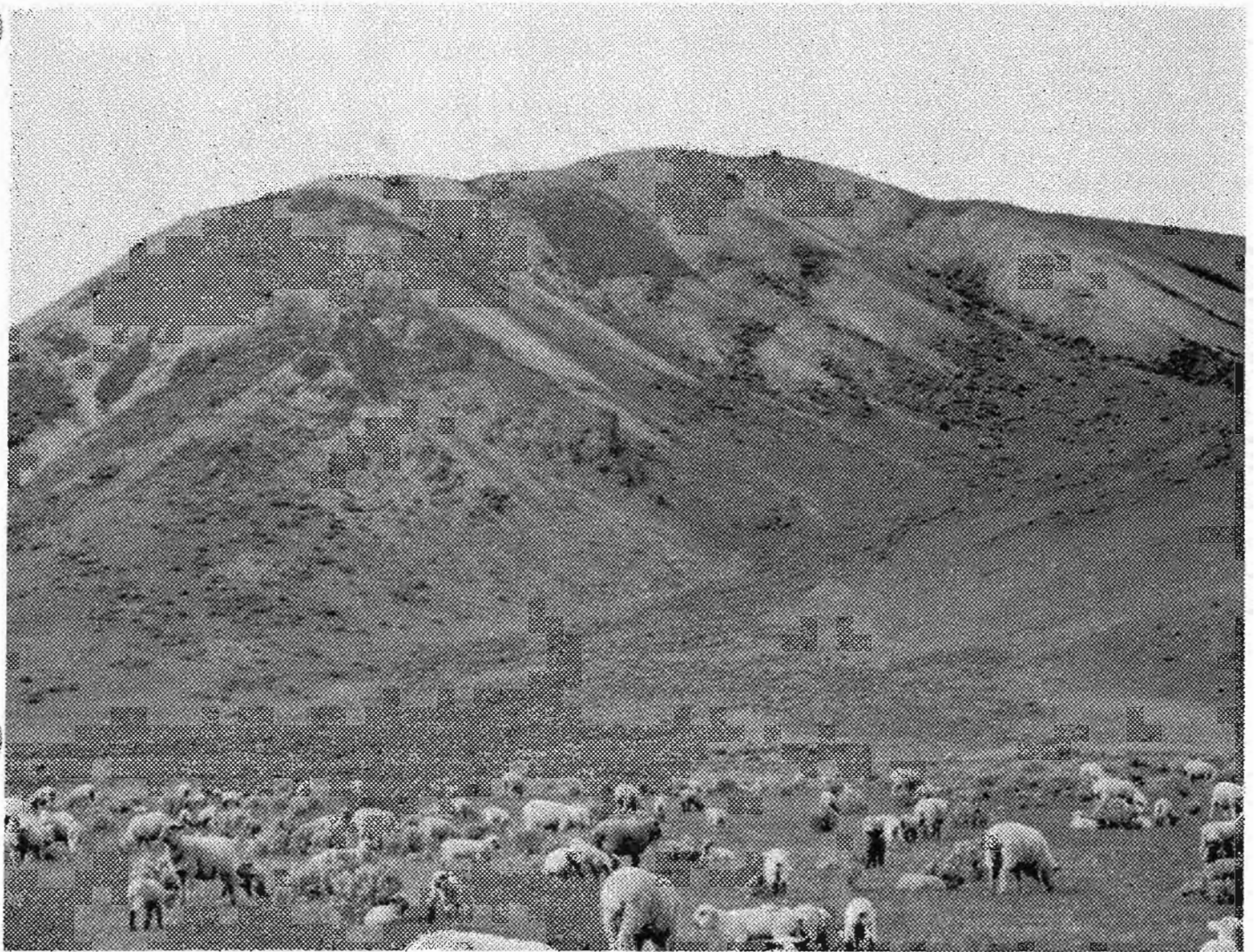
Figure 5-1.—An alluvial fan, Okanogan County, Wash.
