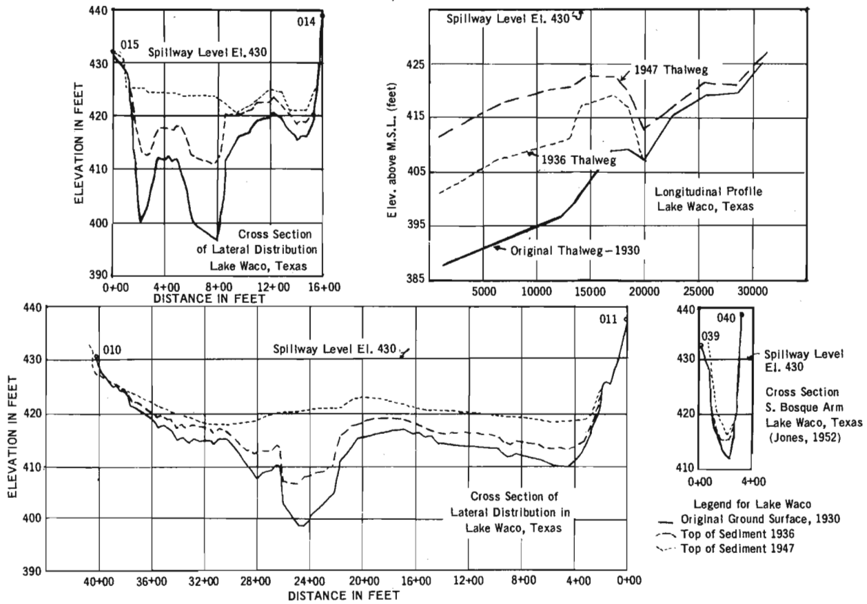
Figure 5-5.—Examples of sediment distribution in reservoirs.
