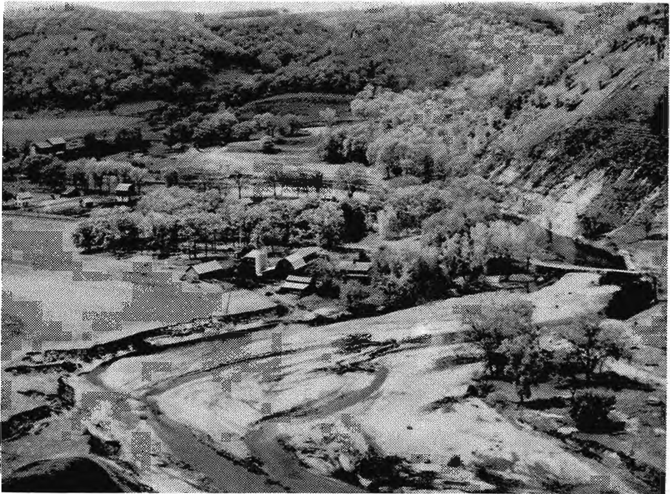
Figure 5-3.—Channel fill, lateral and vertical accretion, Winona County, Minn.
