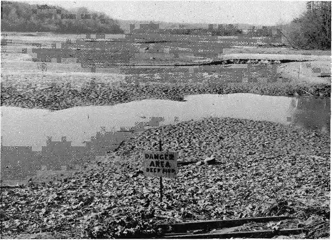
Figure 5-6.—Reservoir sediment accumulation, Lake Accotink, Fairfax County, Va.
