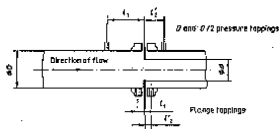
Figure 14-5 -- Flange and D - D/2 pressure taps for orifice meter.
