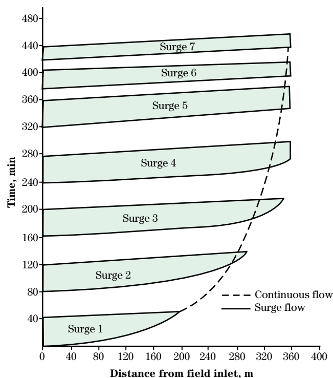
Figure 4-16 Advance and recession trajectories for a surge flow system
