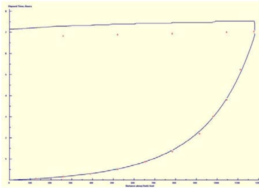
Figure 4–30 Typical advance/recession plot from the Surface graphics output
