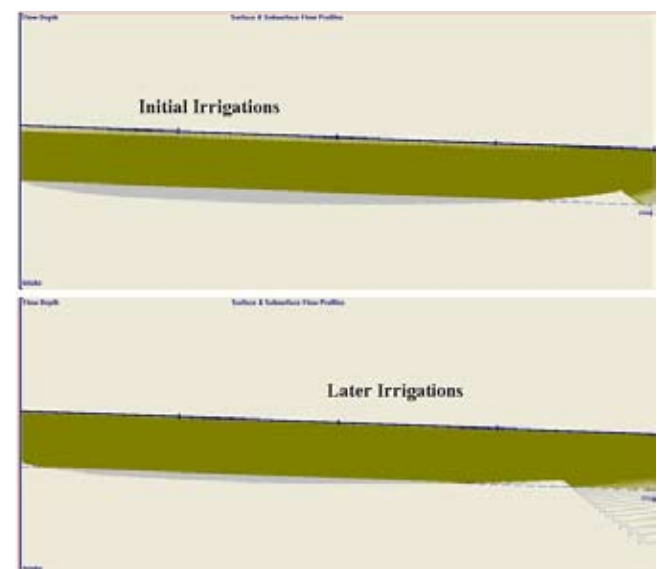
Figure 4-61 Simulation of the BlockedEndBorder.cfg data
