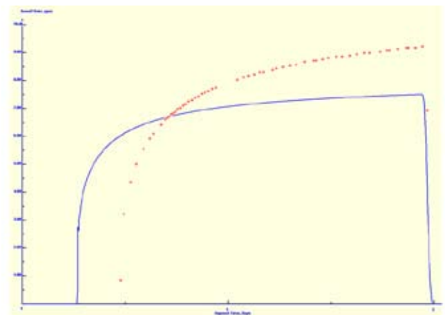
Figure 4–48 Tailwater hydrograph for the example FreeDrainingFurrow_2.cfg data
