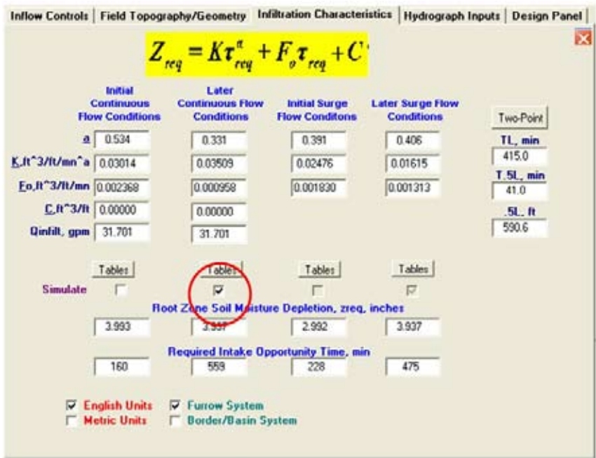
Figure 4–56 Selecting the later irrigation conditions
