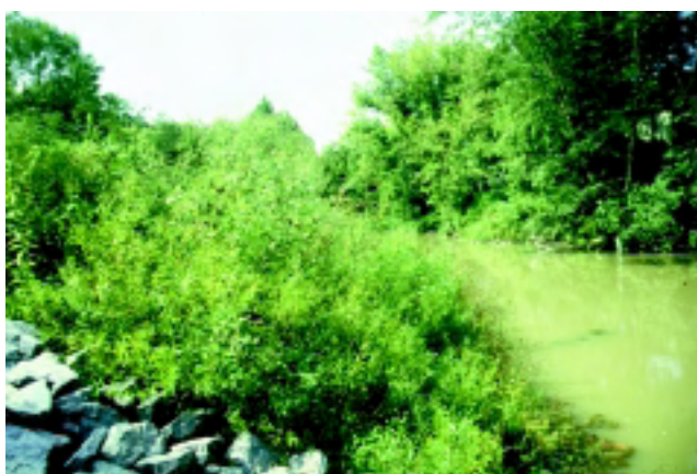
Figure 16-19d Brushmattress system 2 years after installation (Robbin B. Sotir & Associates photo)
