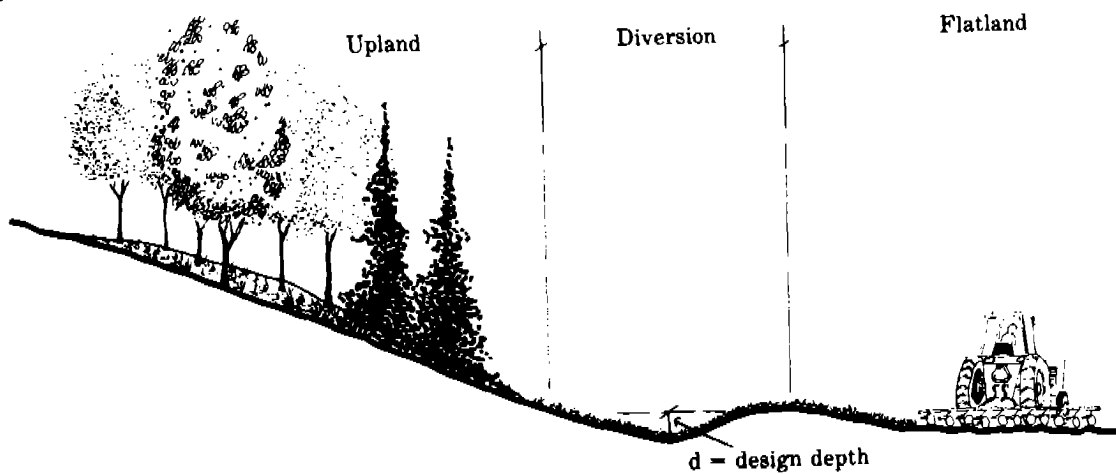
Figure 9-4.—Diversion at base of upland slope.
