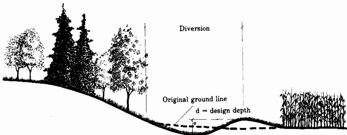
Figure 9-7.—Combination diversion.
