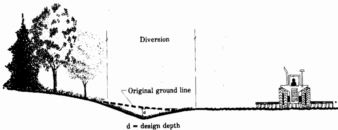
Figure 9-6.—Channel diversion.
