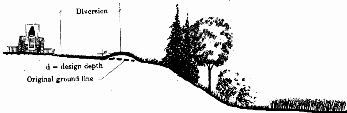
Figure 9-5.—Ridge diversion.
