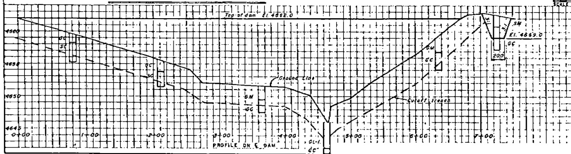
Figure 5-4 Example drawing using plan-profile paper
