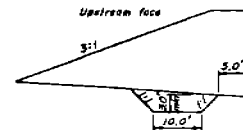
CUTOFF TRENCH DETAIL
