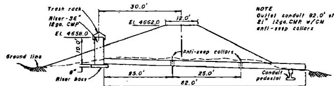
CROSS SECTION THROUGH OUTLET CONDUIT
