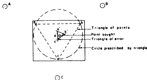
Figure 1-39.—Triangle of error and geometric relationship to point sought (planetable).
