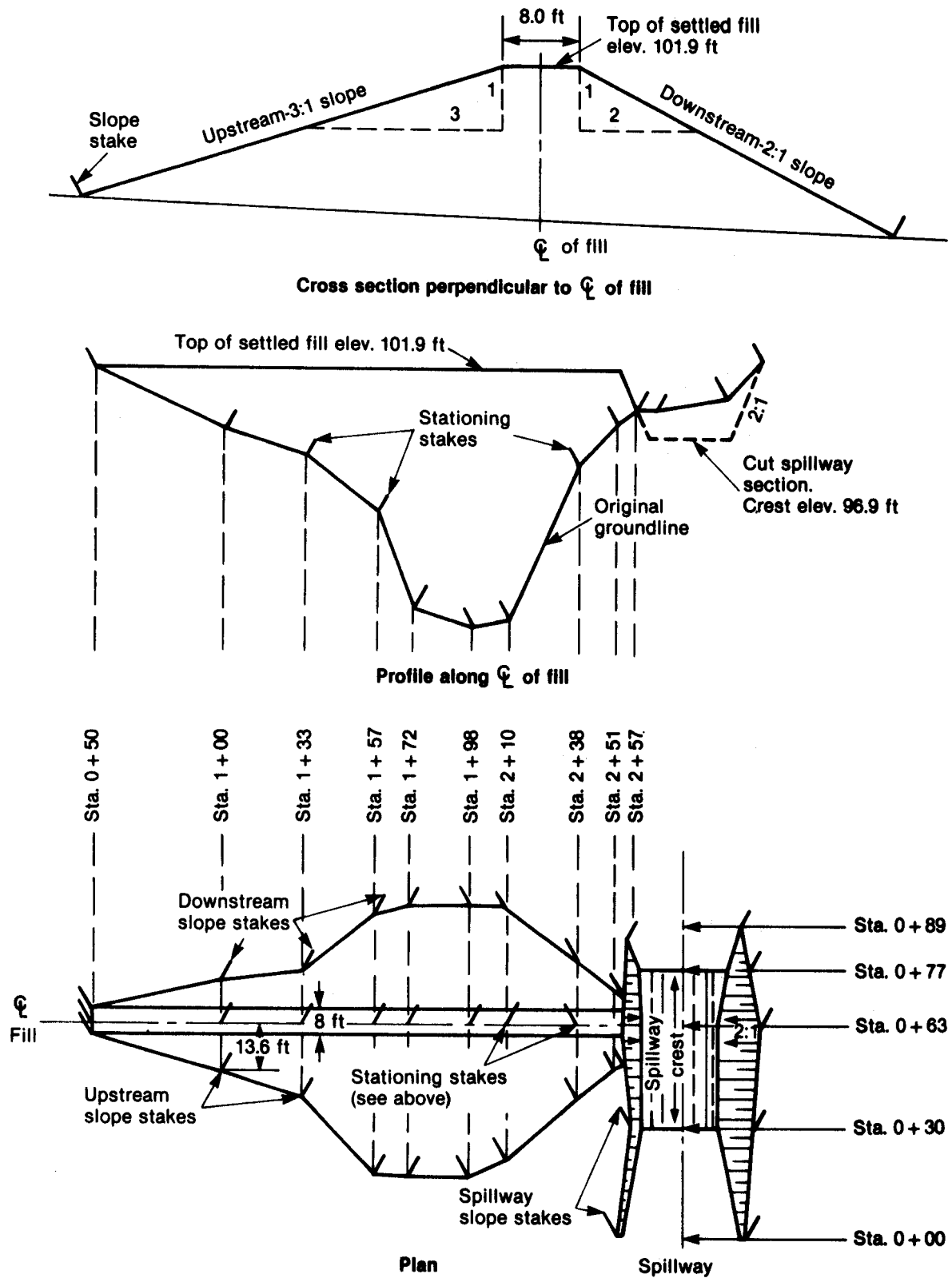
Figure 1-26(a).—Location of slope stakes (English).
