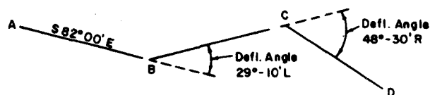
Figure 1-31.—Deflection angles.
