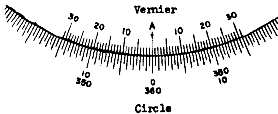
Figure 1-28.—One-minute vernier set at 0°.
