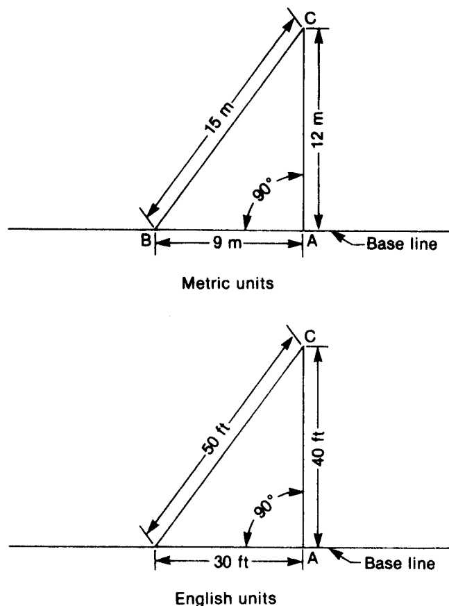
Figure 1-35.—Method 3, 4, and 5 of laying out a right angle.
