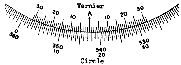
Figure 1-29.—One-minute vernier set for measurement.
