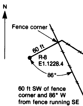
Figure 1-41(a).—Examples—identification of ground control points for stereoplotter (English).
