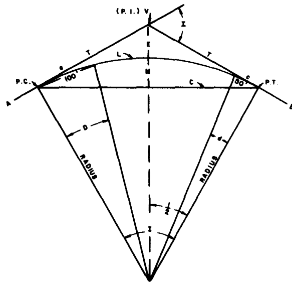
Figure 1-43.—Elements of circular curve.
