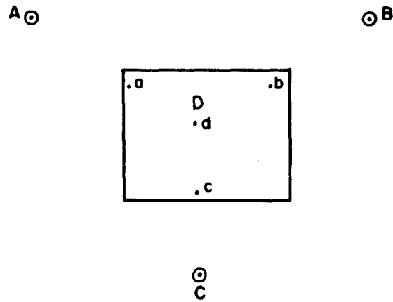
Figure 1-38.—Location of a point on planetable.
