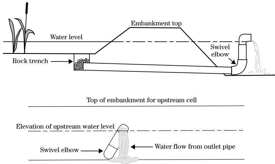
Figure 3-13 Typical configuration of a water-level control structure
