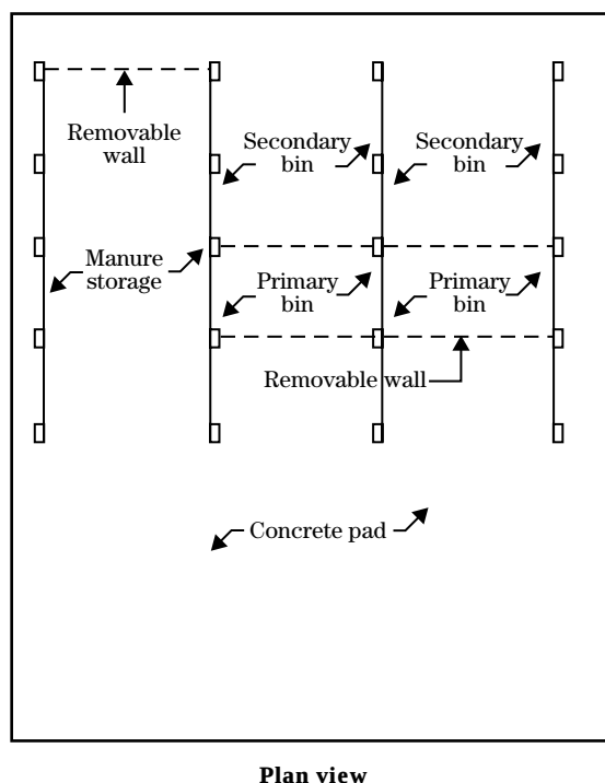
Figure 2–14 Dead bird composter
