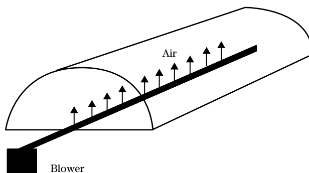
Figure 2-9 Aerated static pile
