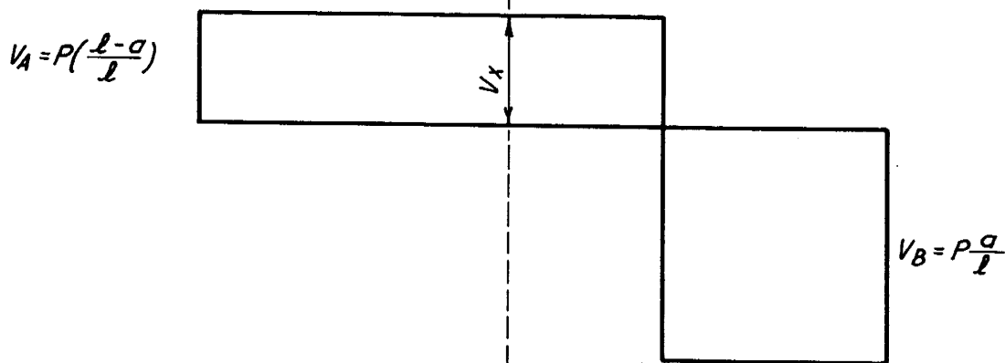
SHEAR DIAGRAM
