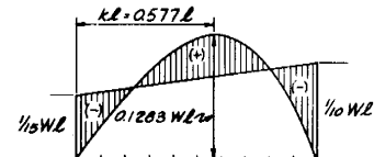
Moment Diagram
