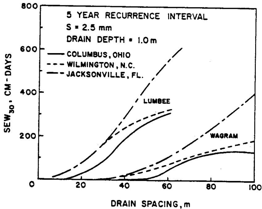
Figure 6-9. SEW-30 versus drain spacing for Lumbée and Wagram soils at all three locations.
