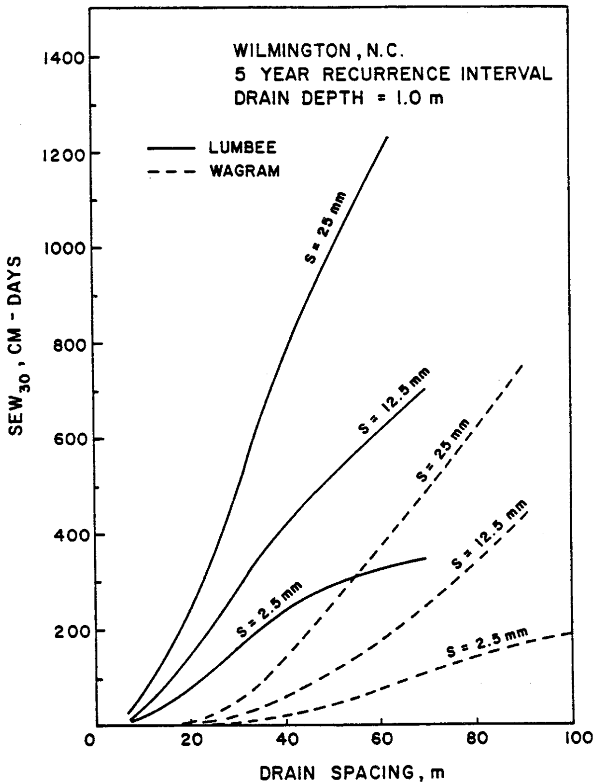
Figure 6-6. SEW-30 versus drain spacing for 3 levels of surface drainage on Lumbee and Wagram soils at Wilmington, North Carolina.
