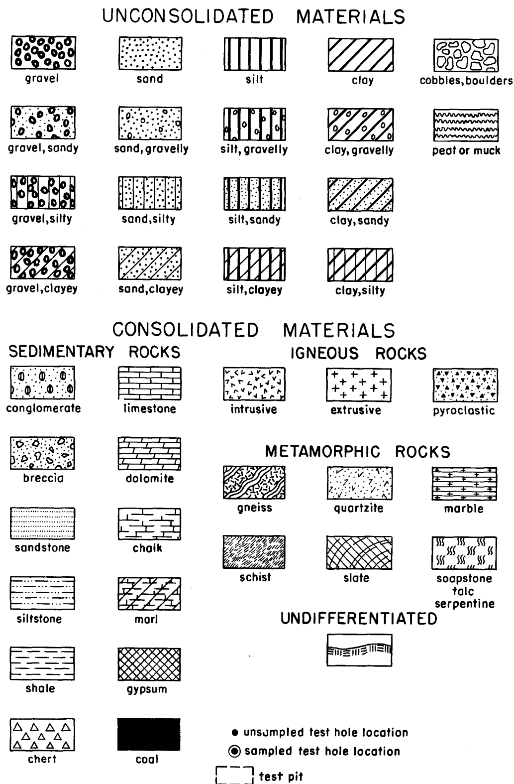
Figure 1-3. Standard SCS Geologic Symbols
