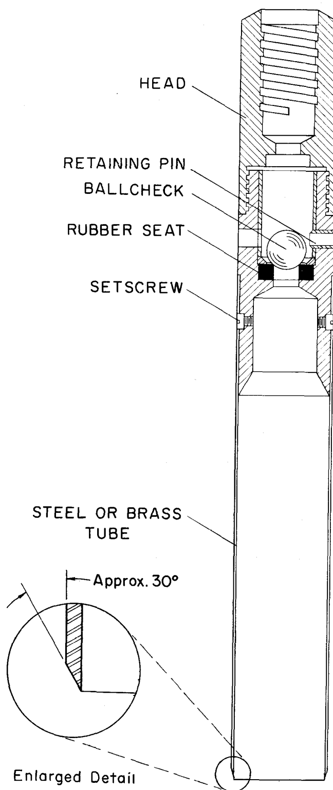
Figure 2-14 Thin-wall Open Drive Sampler
