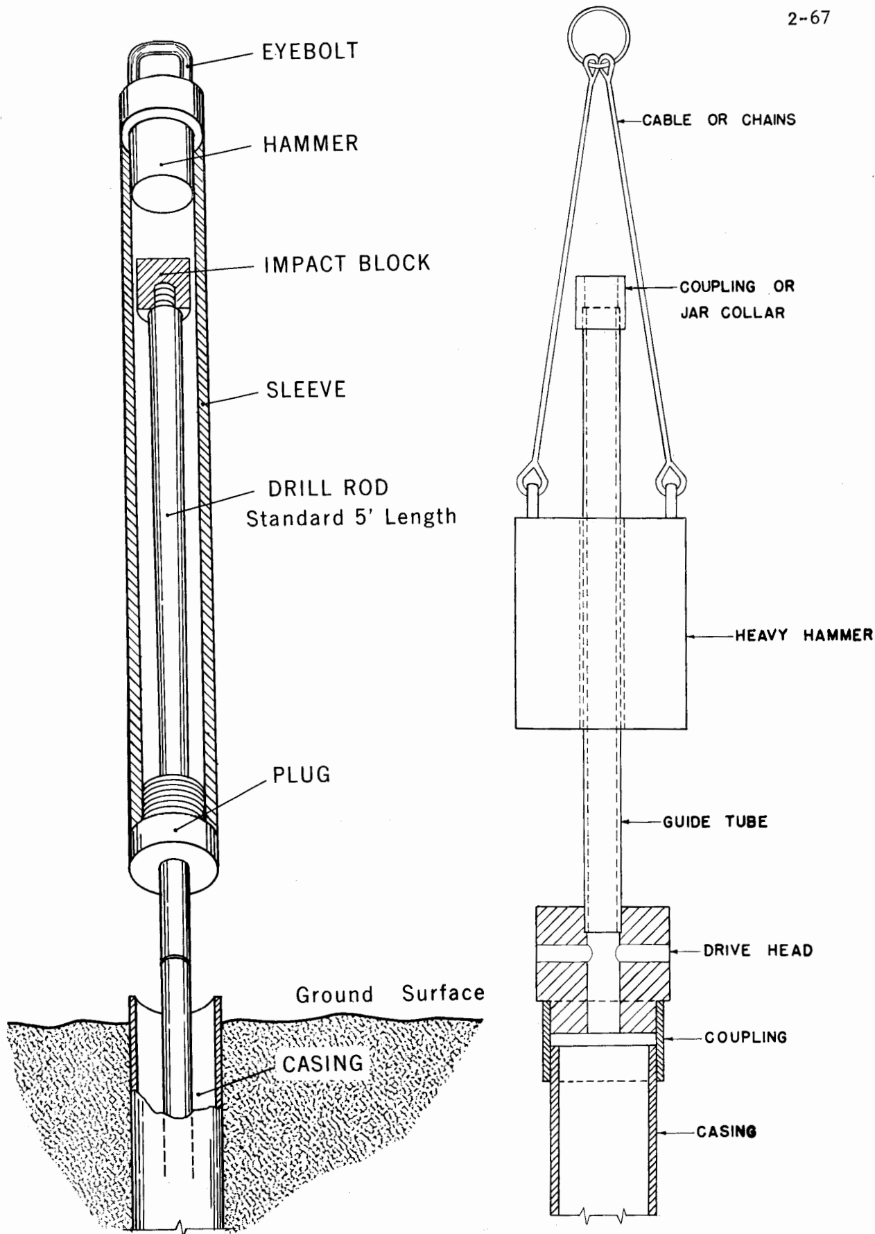
Figure 2-23 Safety and Casing Drive Hammers
