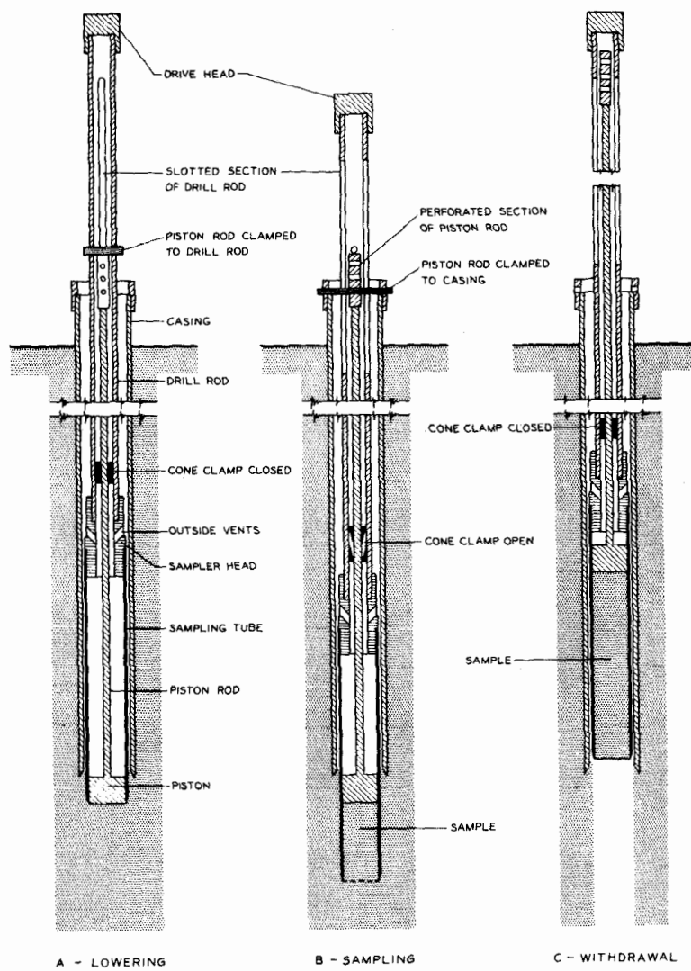
Figure 2-15 Stationary-Piston Sampler
