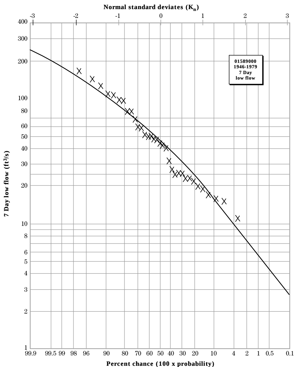
Figure 18-2 Data and frequency curve for example 18-2
