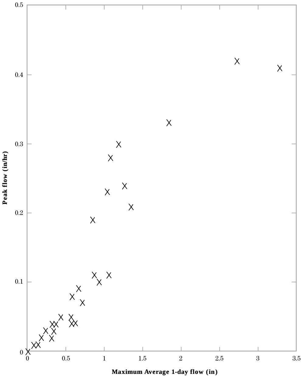
Figure 18-10 Variable plot for example 18-4
