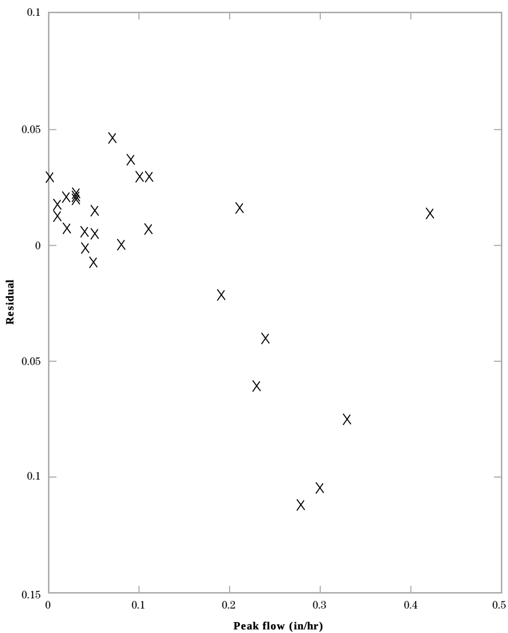
Figure 18-11 Residual plot for example 18-4
