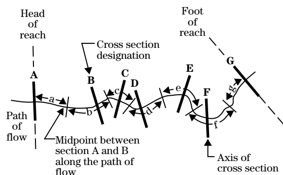
Figure 13-3 Flood damage reach showing weighting of area between cross sections
