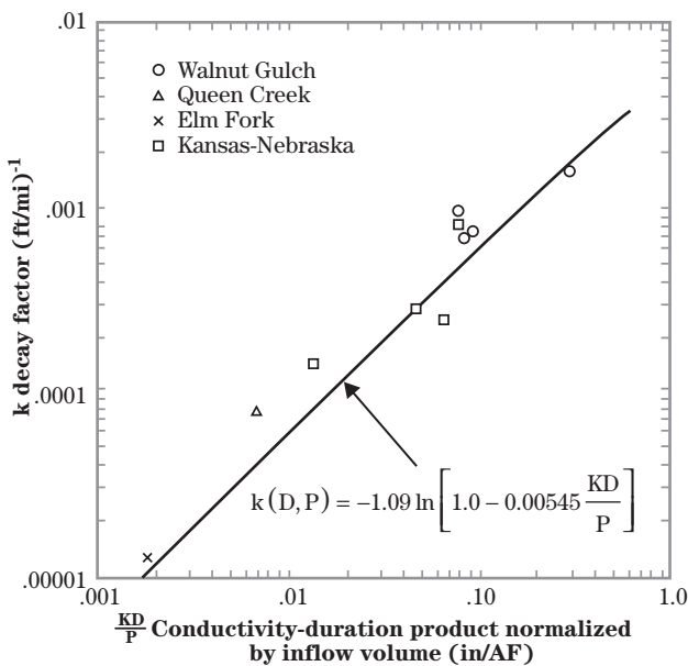
Figure 19C-2 Relation between KD/P and decay factor
