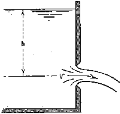
Figure 2-2a -- Orifice flow.
