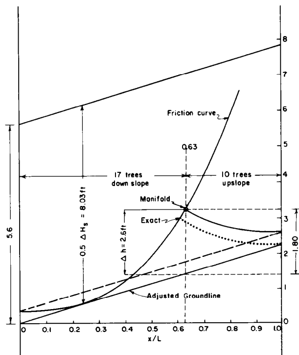
Figure 7-46.—Friction curve overlay to demonstrate graphical solution of manifold positioning and \Delta h (difference in pressure head along the lateral). \Delta H_s = allowable subunit pressure-head variation; x = position of manifold along lateral; L = length of lateral.
