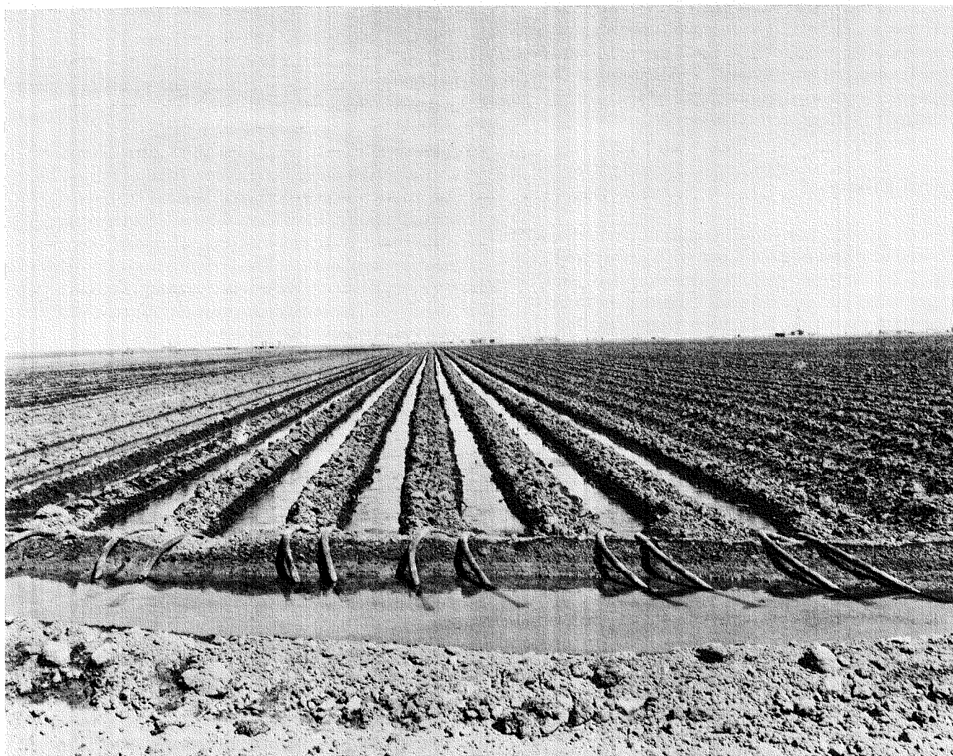
Figure 5-2.—Level furrow irrigation.
