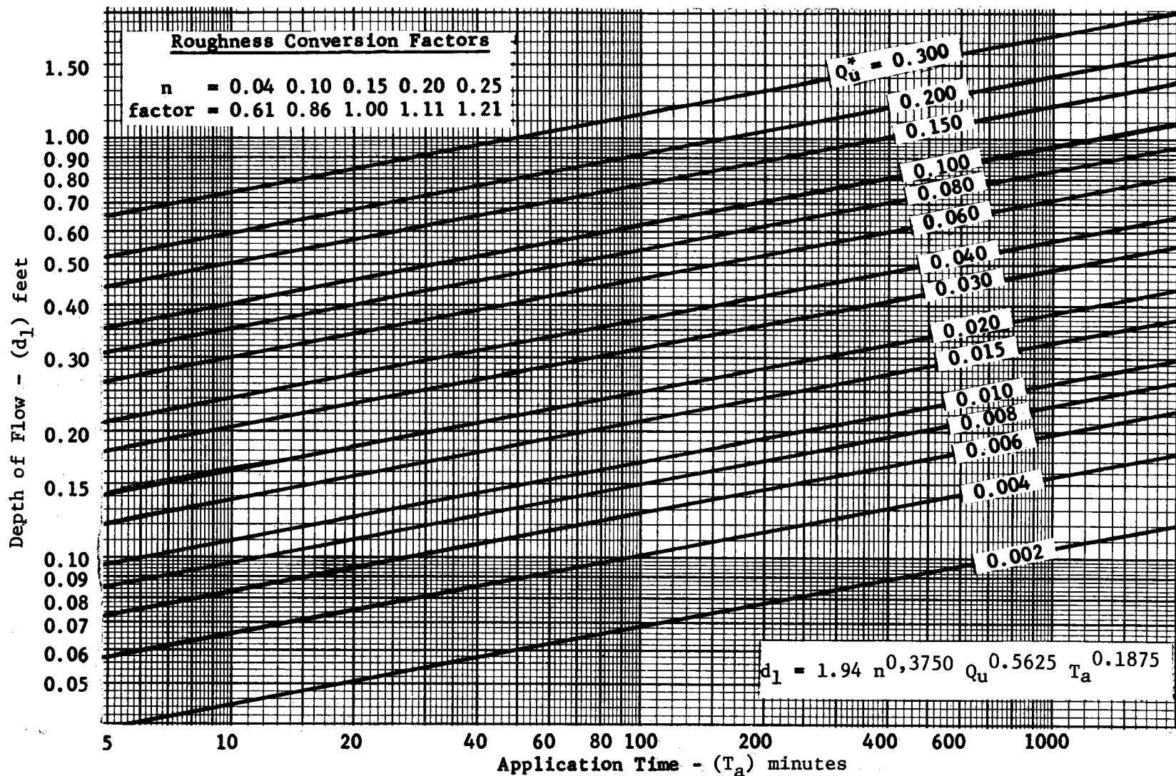
Figure 4-4.---Chart for estimating depth of flow in level borders with n of 0.15
