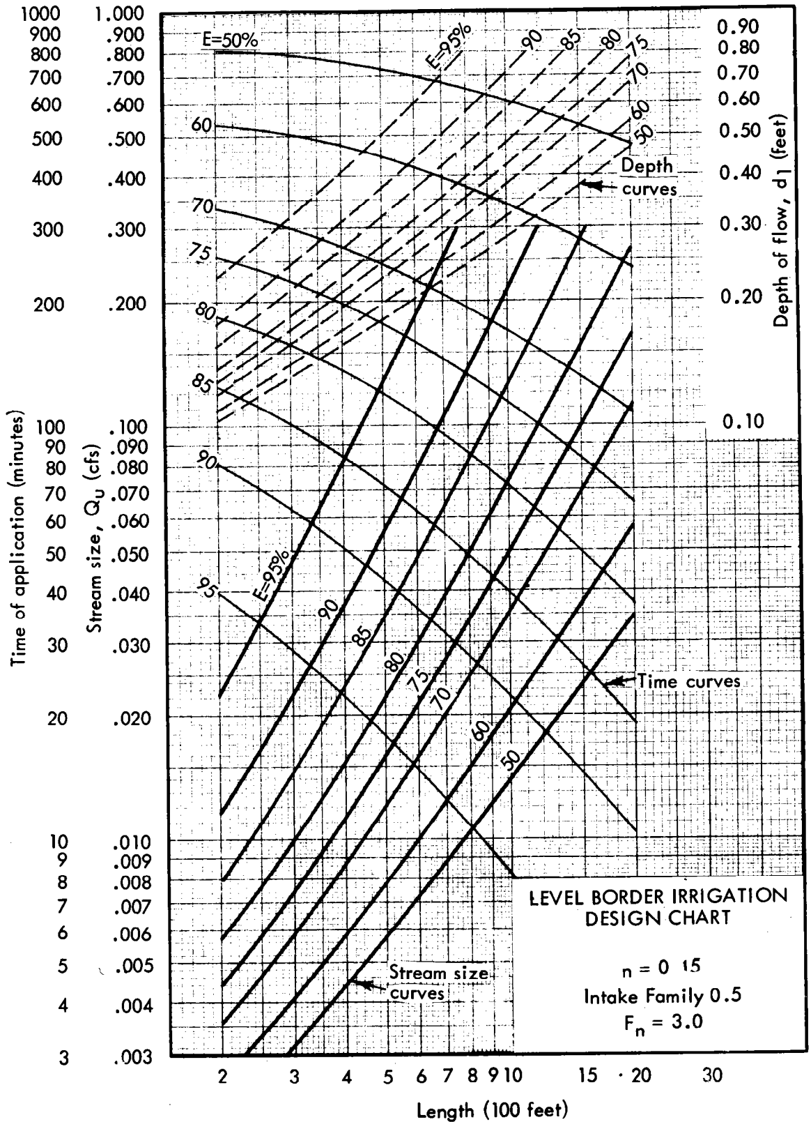
Figure 4-5.--Sample design chart for level border irrigation.
