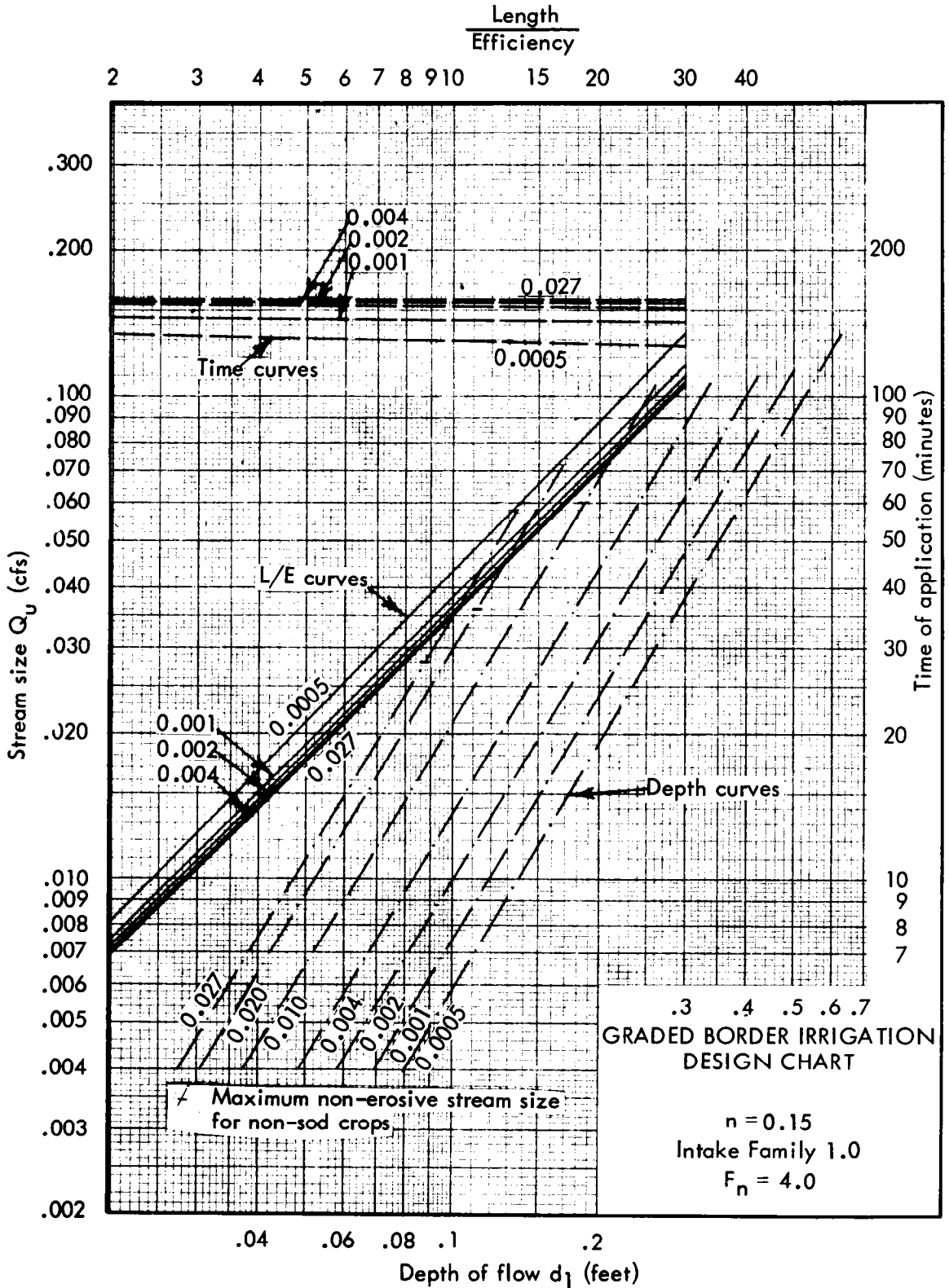
Figure 4-8.--Sample design chart for graded border irrigation
