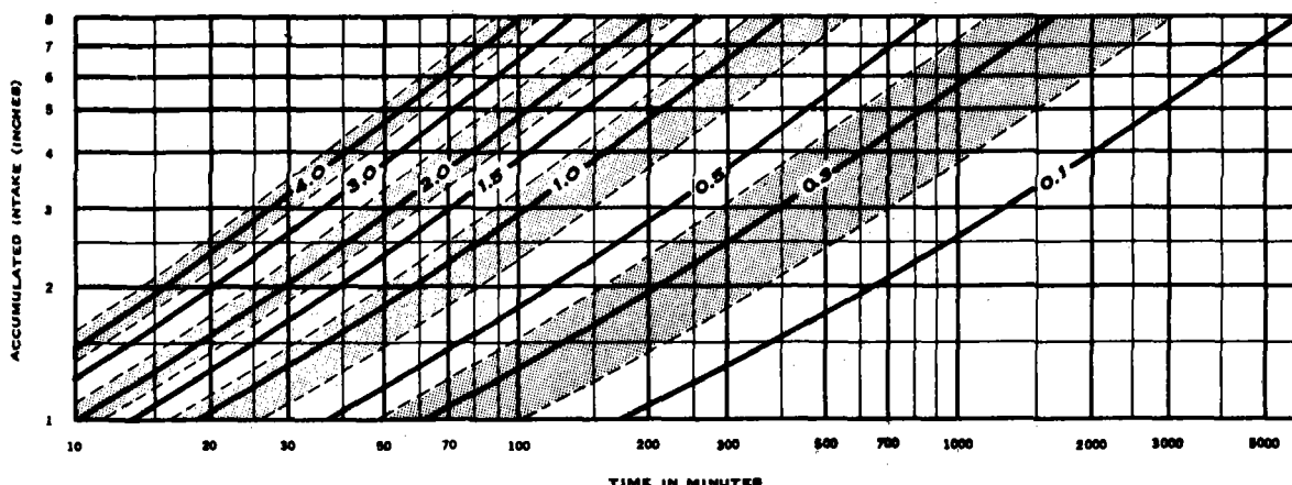
Figure 4-1.--Intake families for border irrigation design
