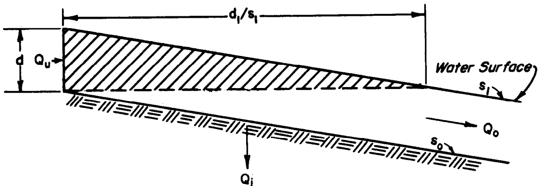
Figure 4-6.--Diagram of recession-lag time
