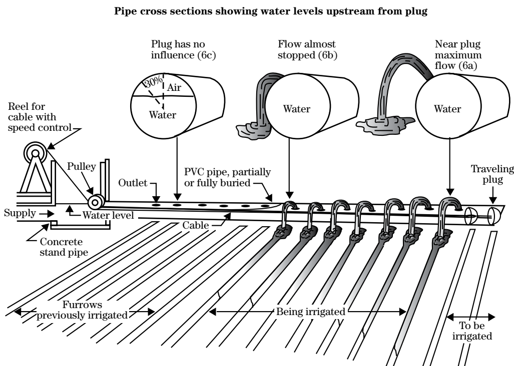
Figure 4-15 Schematic cablegation system
