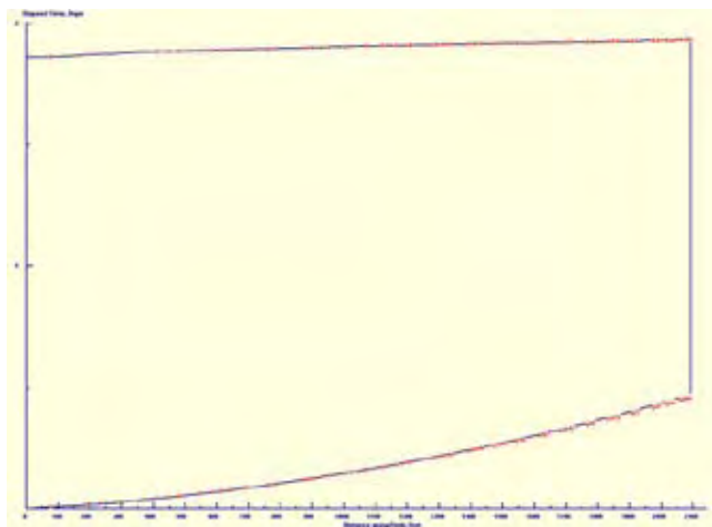
Figure 4-49 Corrected advance/recession curve for FreeDrainingFurrow_2.cfg data
