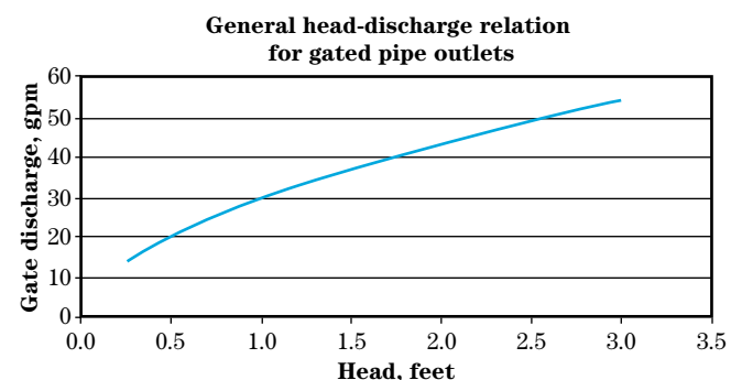
Figure 4-69 Typical head-discharge curve for gated pipe outlets
