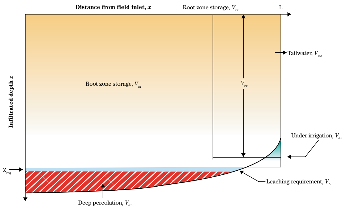
Figure 4–42 Distribution of applied water in surface irrigation
