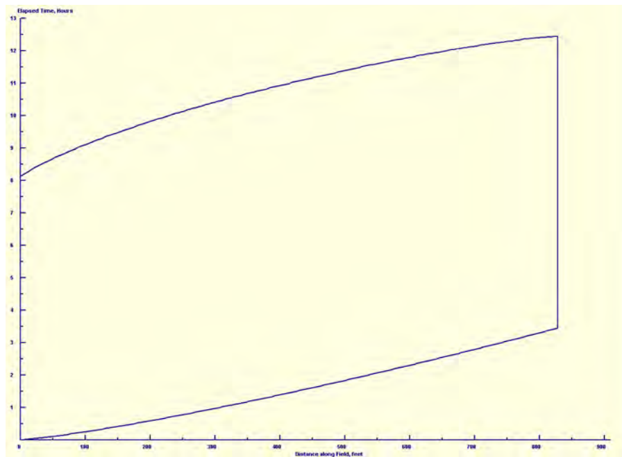
Figure 4-57 FreeDrainingBorder_4 advance and recession plots for initial irrigations
