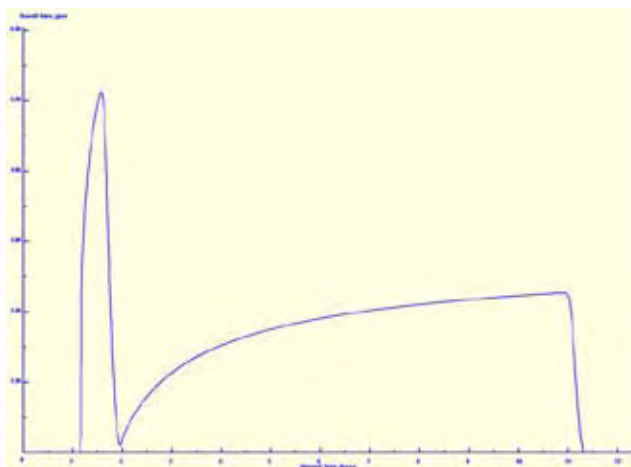
Figure 4–62 Simulated tailwater hydrograph using the CutbackDesign.cfg data file
