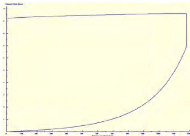
Figure 4–51 FreeDrainingFurrow_1 advance/recession trajectory
