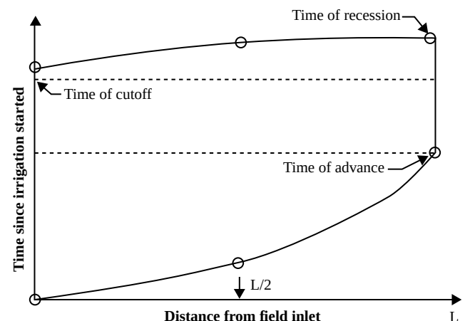
Figure 4-45 Field measurement points for advance and recession evaluations in the field
