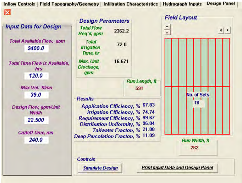
Figure 4–55 Improved design for initial irrigations
