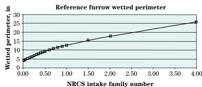
Figure 4–40 Reference furrow wetted perimeters for the revised NRCS intake families
