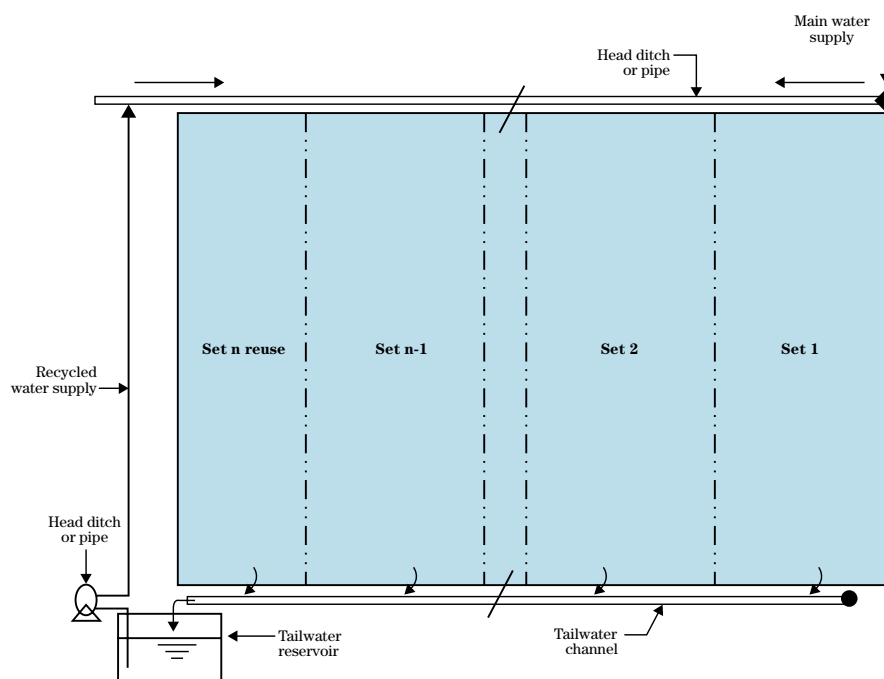
Figure 4-63 Schematic tailwater reuse system
