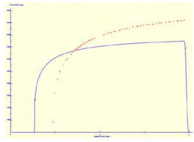
Figure 4–48 Tailwater hydrograph for the example FreeDrainingFurrow_2.cfg data
