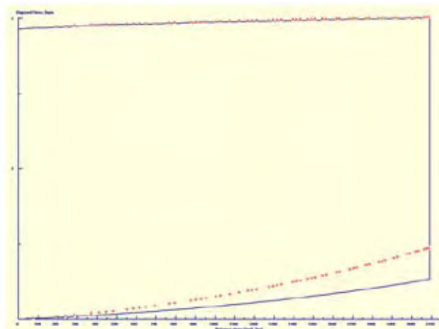
Figure 4–47 Advance/recession curve for the example FreeDrainingFurrow_2.cfg data
