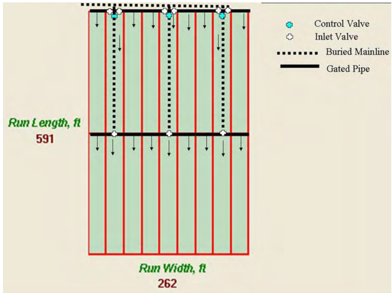
Figure 4–71 Alternative gated pipe layout for FreeDrainingFurrow_1.cfg
