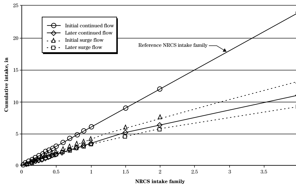
Figure 4–39 Average 6-hour intake rate for the revised NRCS furrow intake families
