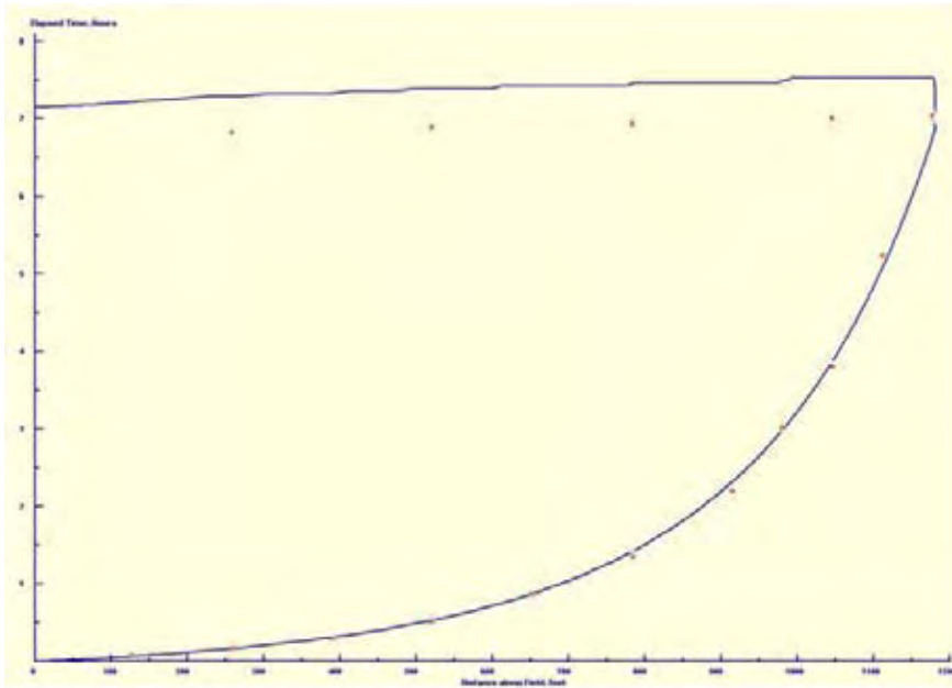
Figure 4–30 Typical advance/recession plot from the Surface graphics output
