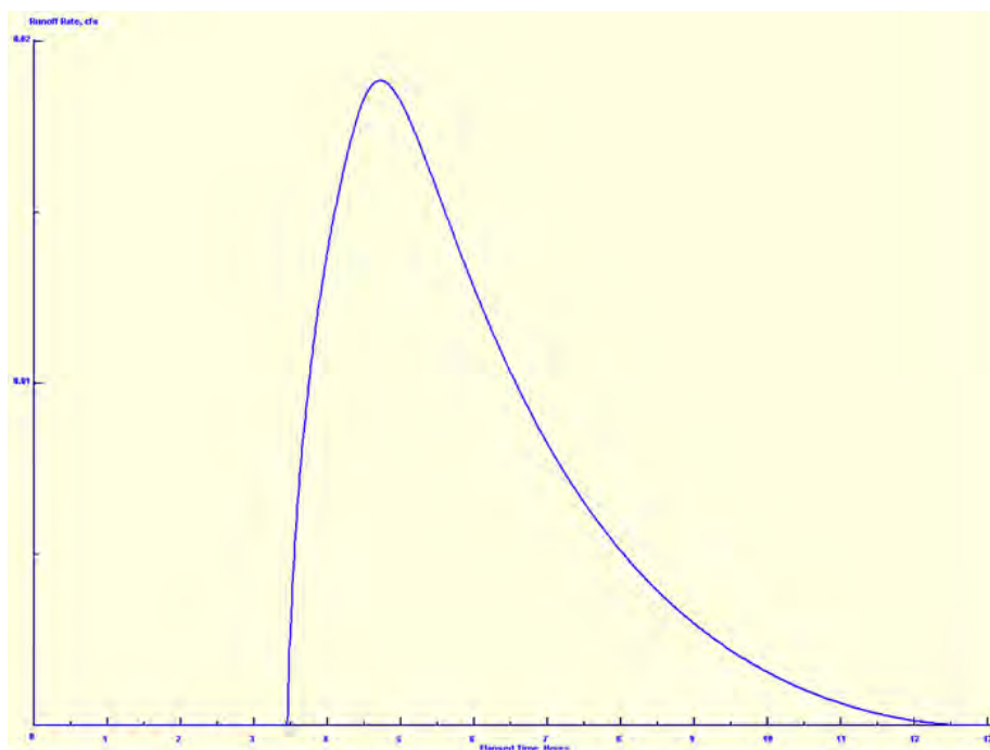
Figure 4-58 Tailwater hydrograph for FreeDrainingBorder_4 data
