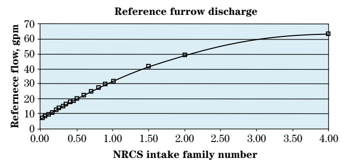
Figure 4–41 Relationship of reference flow to intake family
