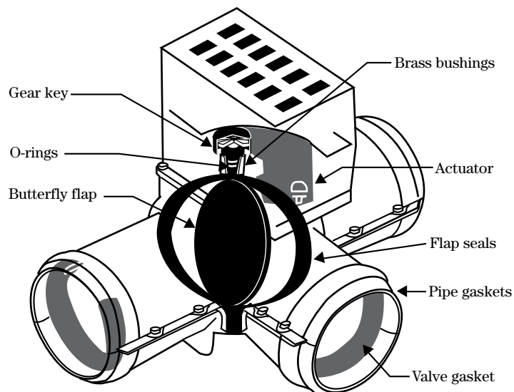
Figure 4-18 Automated butterfly surge flow valve
