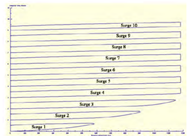
Figure 4–65 Surge flow advance and recession plot for FreeDrainingFurrow_1Surge example
