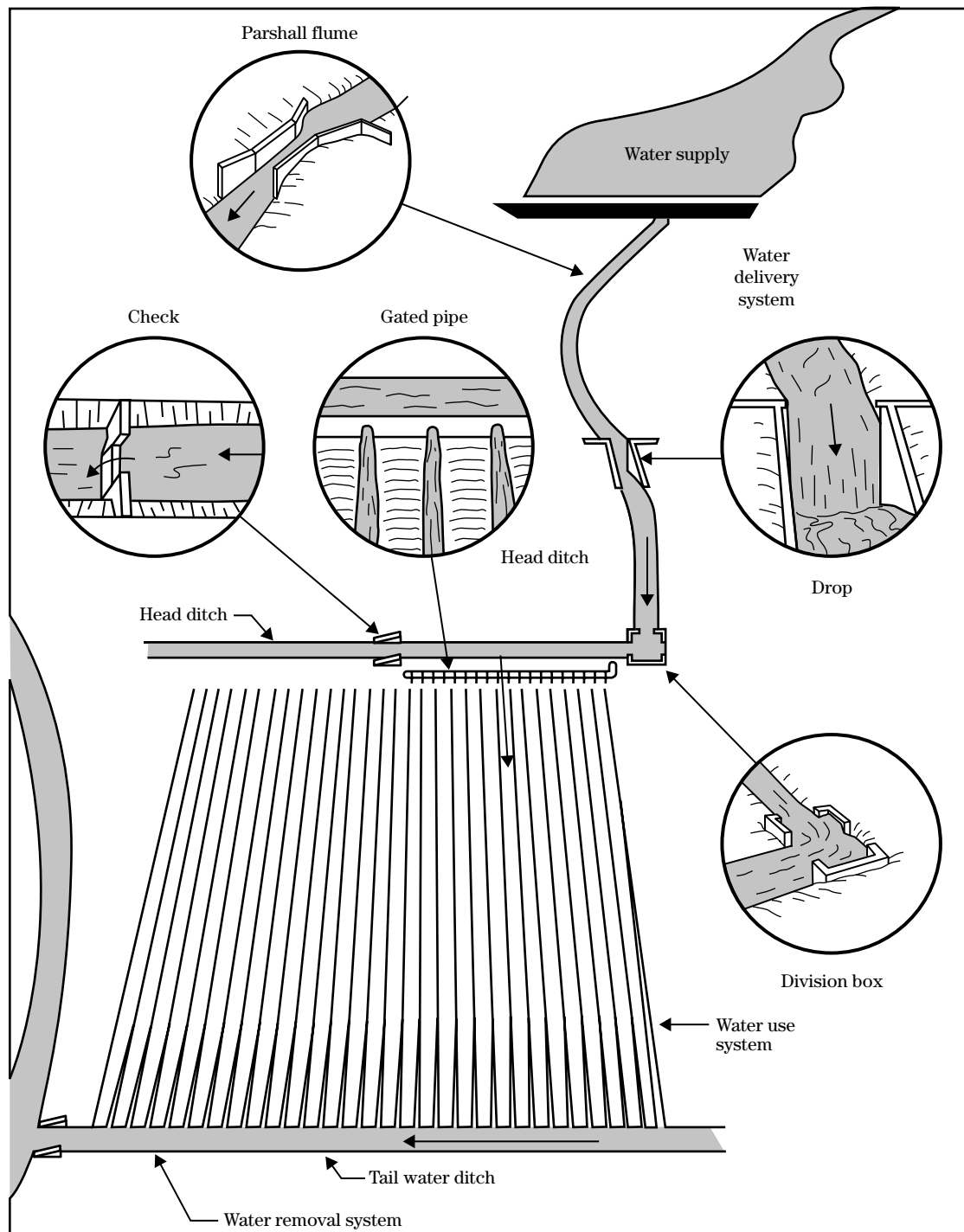
Figure 4-1 Layout and function of irrigation system components
