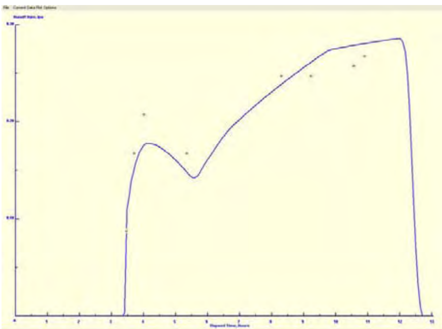
Figure 4–31 Typical runoff hydrograph from the Surface graphic output
