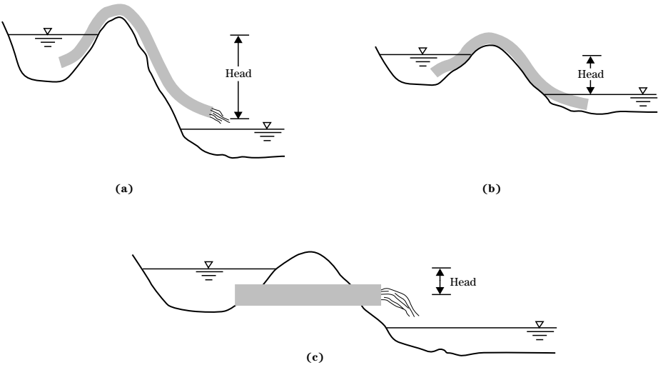
Figure 4-68 Typical operational conditions of surface irrigation siphons and spiles
