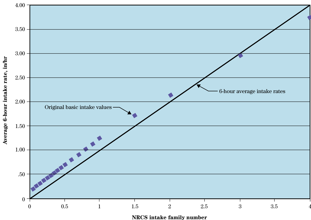
Figure A-1 Comparison between the average 6-hour intake rate and the basic intake rate of the original SCS intake families
