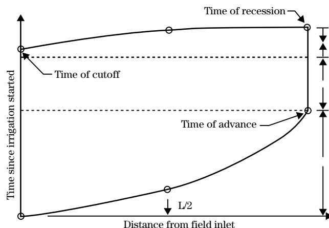
Figure 4–2 Basic phases of a surface irrigation event
