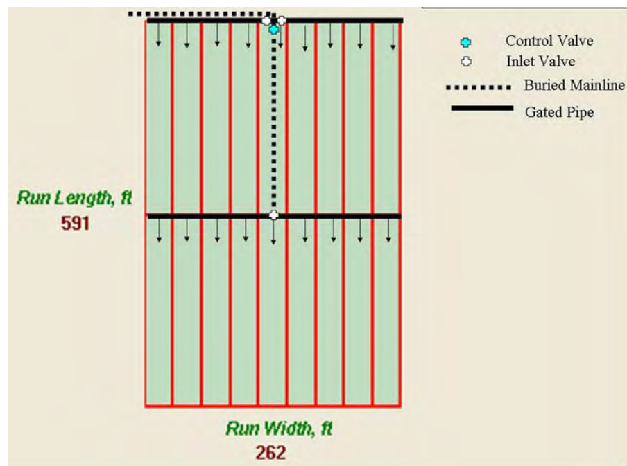
Figure 4–70 Layout of FreeDrainingFurrow_1 gated pipe system
