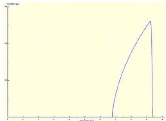
Figure 4–52 FreeDrainingFurrow_1 tailwater hydrograph
