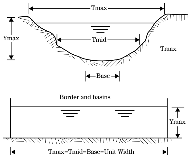
Figure 4-43 Cross-sectional shapes for furrow and border/basin irrigation
