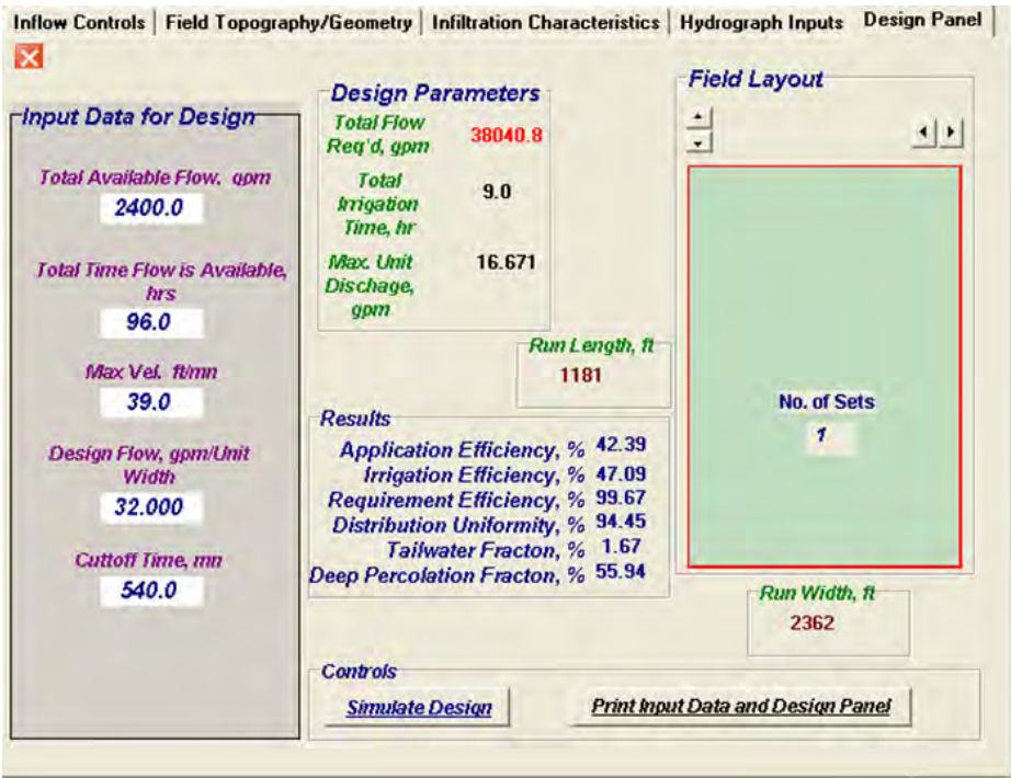
Figure 4–54 Surface Design Panel for initial FreeDrainingFurrow_1 condition
