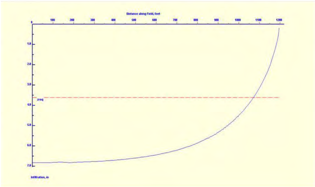
Figure 4–32 Typical plot of intake distribution for the Surface graphics output
