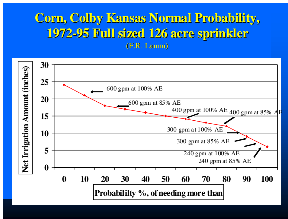
Figure 1. Effect of Irrigation Capacity on Irrigation System Reliability.
