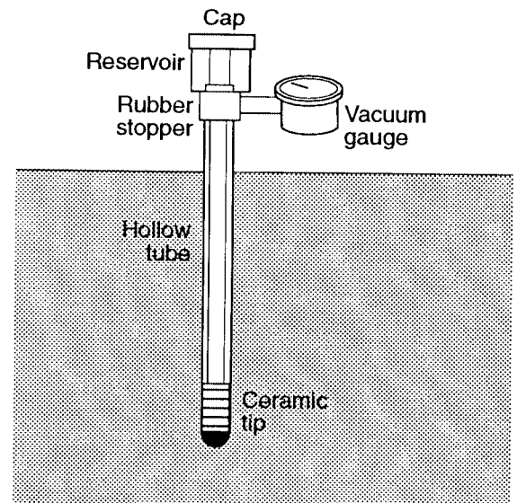
Figure 3. A typical tensiometer.
