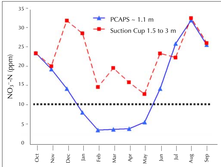
Figure 1. Measured monthly average \text{NO}_3^- -N (nitrogen as nitrate) concentrations below seven Lane County mint fields during the 5-year study period. Concentrations were measured by passive capillary samplers (PCAPS) as well as by suction cup samplers. The dotted line indicates the EPA drinking water standard of 10 ppm \text{NO}_3^- -N (from Feaga and Selker, 2004).
