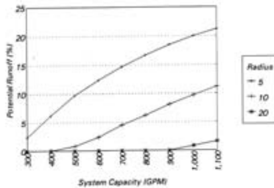
Figure 11. Predicted Irrigation Runoff Potential for Various System Capacities and Wetted Radius. Storage – 0.5 in.; App. Amt. – 1.0 in.; Intake Family – 0.3; System Length – 1,280 ft.
