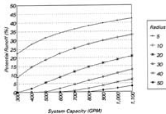
Figure 12. Predicted Irrigation Runoff Potential for Various System Capacities and Wetted Radius. Storage – 0.5 in.; App. Amt. – 1.5 in.; Intake Family – 0.3; System Length – 1,280 ft.
