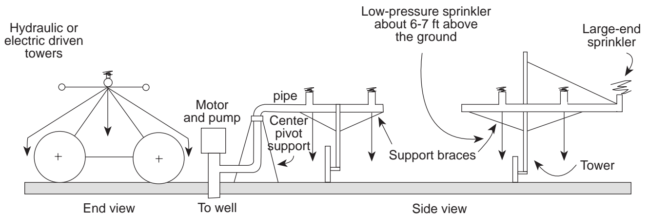
Figure 2. Mechanical-move sprinkler system: Self-propelled (center-pivot) lateral.
