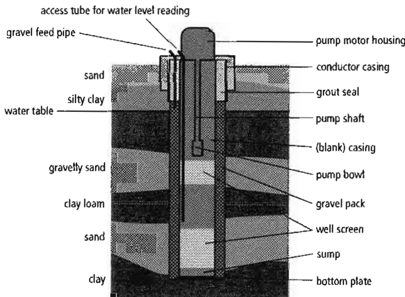
Figure 1. Components of a well.
