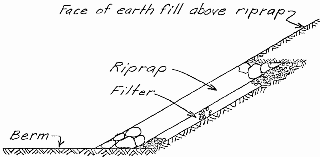
(a) UNACCEPTABLE DETAIL
