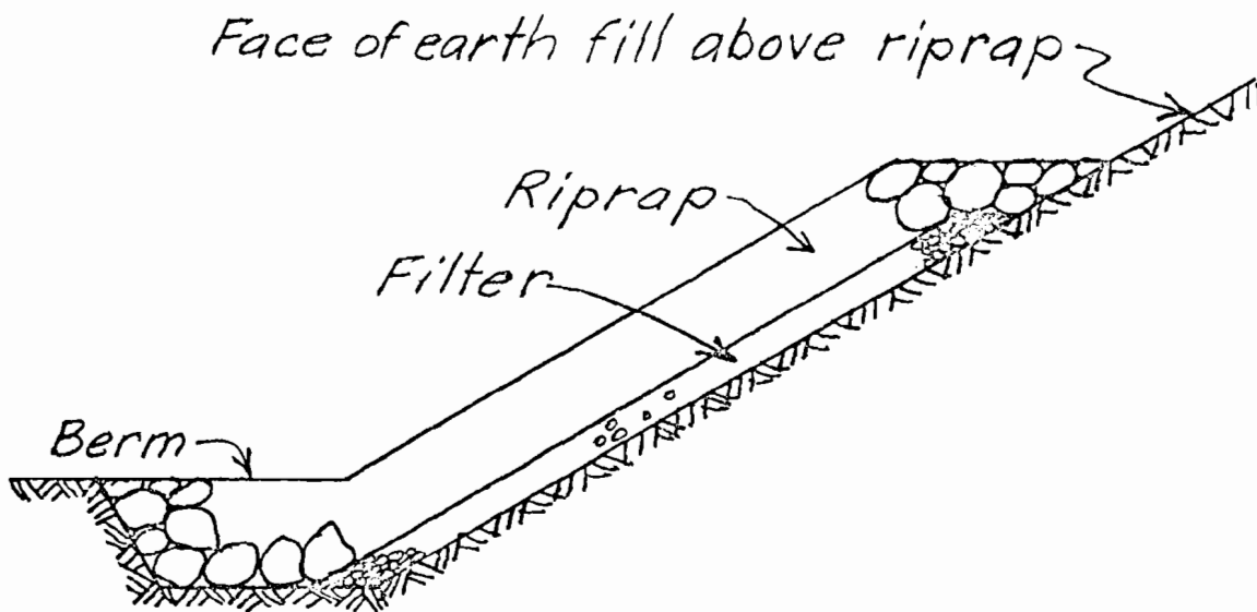
(b) ACCEPTABLE DETAIL
