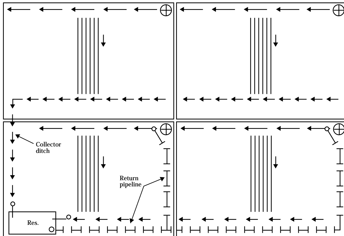
Figure 6-6 Typical layout for a tailwater recovery and reuse facility
