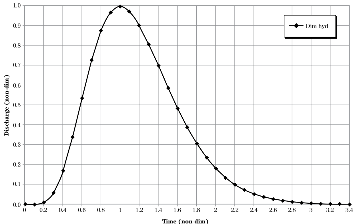
Figure 16B-1 Peak rate factor = 600
