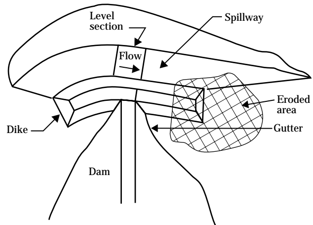
Figure 50-4 Spillway gully resulting in breach of spillway
