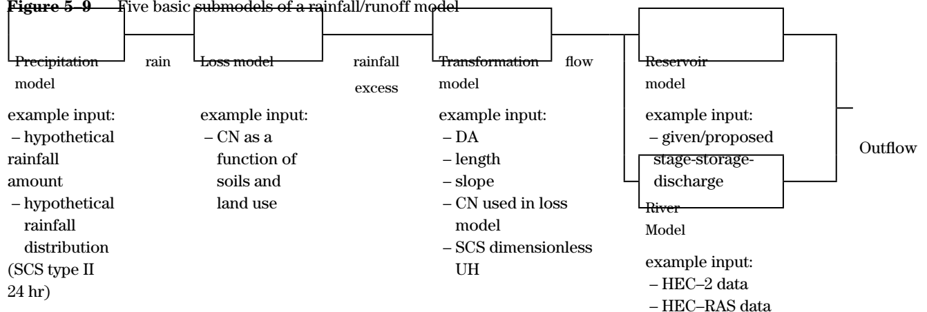
Figure 5-9 Five basic submodels of a rainfall/runoff model
